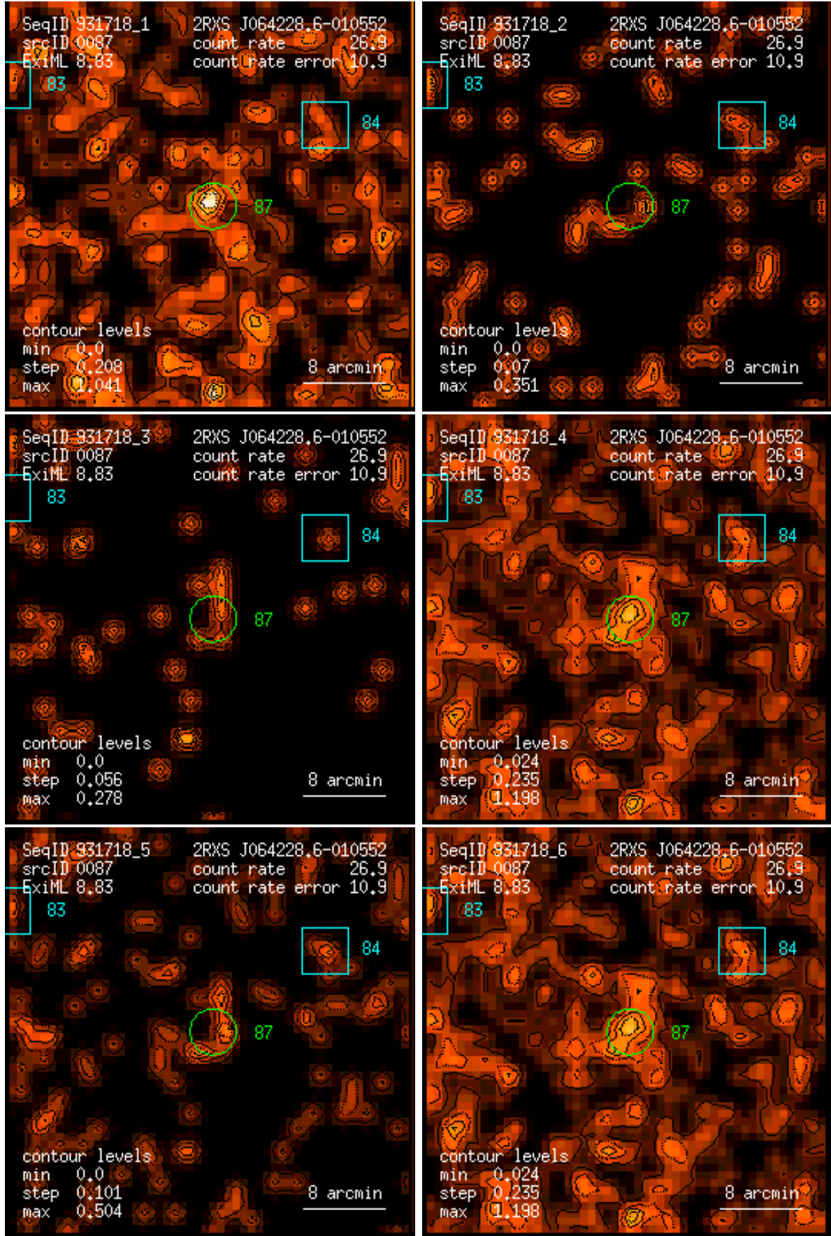
Figure 87: RASS 931718: detection 0087: band rate images, Gaussian filter: (1) PSPC channels 11 – 41, (2) 52 – 90, (3) 91 – 201, (4) 11 – 235, (5) 52 – 201, (6) 11 – 201. Broad band rates in counts/ks. Band rate contour levels in counts/ks/arcmin 2 .
