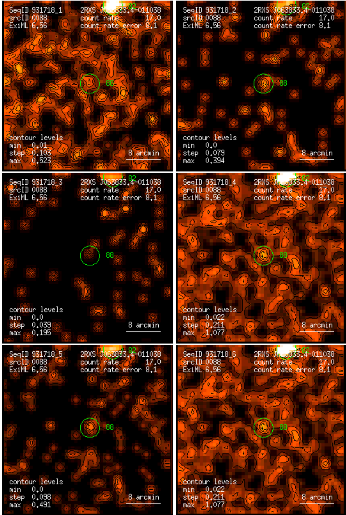
Figure 88: RASS 931718: detection 0088: band rate images, Gaussian filter: (1) PSPC channels 11 – 41, (2) 52 – 90, (3) 91 – 201, (4) 11 – 235, (5) 52 – 201, (6) 11 – 201. Broad band rates in counts/ks. Band rate contour levels in counts/ks/arcmin 2 .
