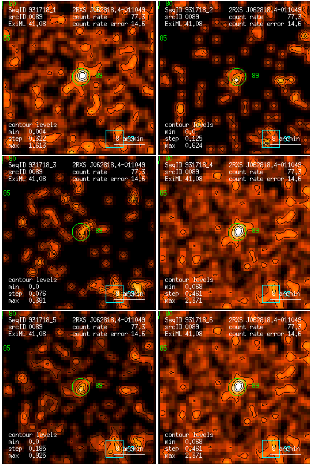
Figure 89: RASS 931718: detection 0089: band rate images, Gaussian filter: (1) PSPC channels 11 – 41, (2) 52 – 90, (3) 91 – 201, (4) 11 – 235, (5) 52 – 201, (6) 11 – 201. Broad band rates in counts/ks. Band rate contour levels in counts/ks/arcmin 2 .
