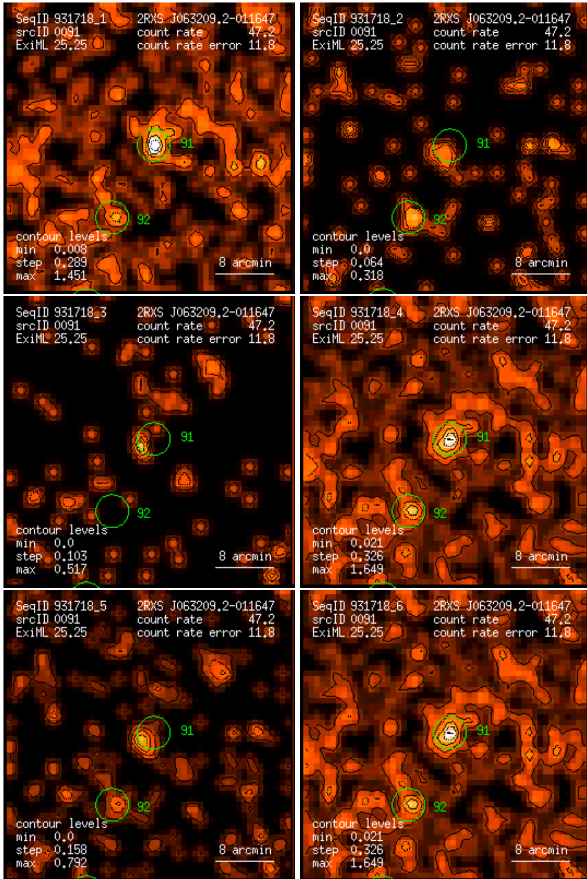
Figure 91: RASS 931718: detection 0091: band rate images, Gaussian filter: (1) PSPC channels 11 – 41, (2) 52 – 90, (3) 91 – 201, (4) 11 – 235, (5) 52 – 201, (6) 11 – 201. Broad band rates in counts/ks. Band rate contour levels in counts/ks/arcmin 2 .
