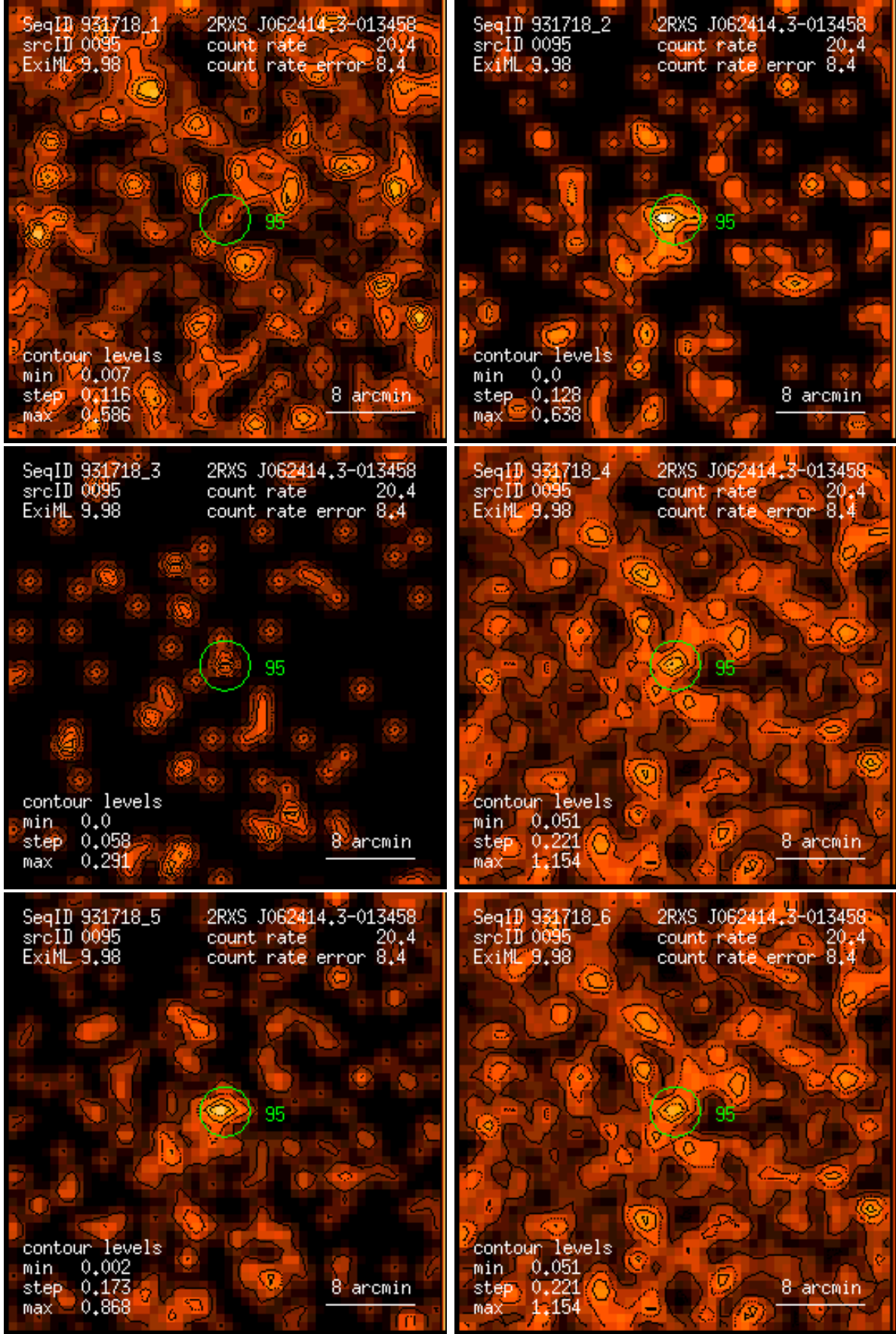
Figure 95: RASS 931718: detection 0095: band rate images, Gaussian filter: (1) PSPC channels 11 – 41, (2) 52 – 90, (3) 91 – 201, (4) 11 – 235, (5) 52 – 201, (6) 11 – 201. Broad band rates in counts/ks. Band rate contour levels in counts/ks/arcmin 2 .
