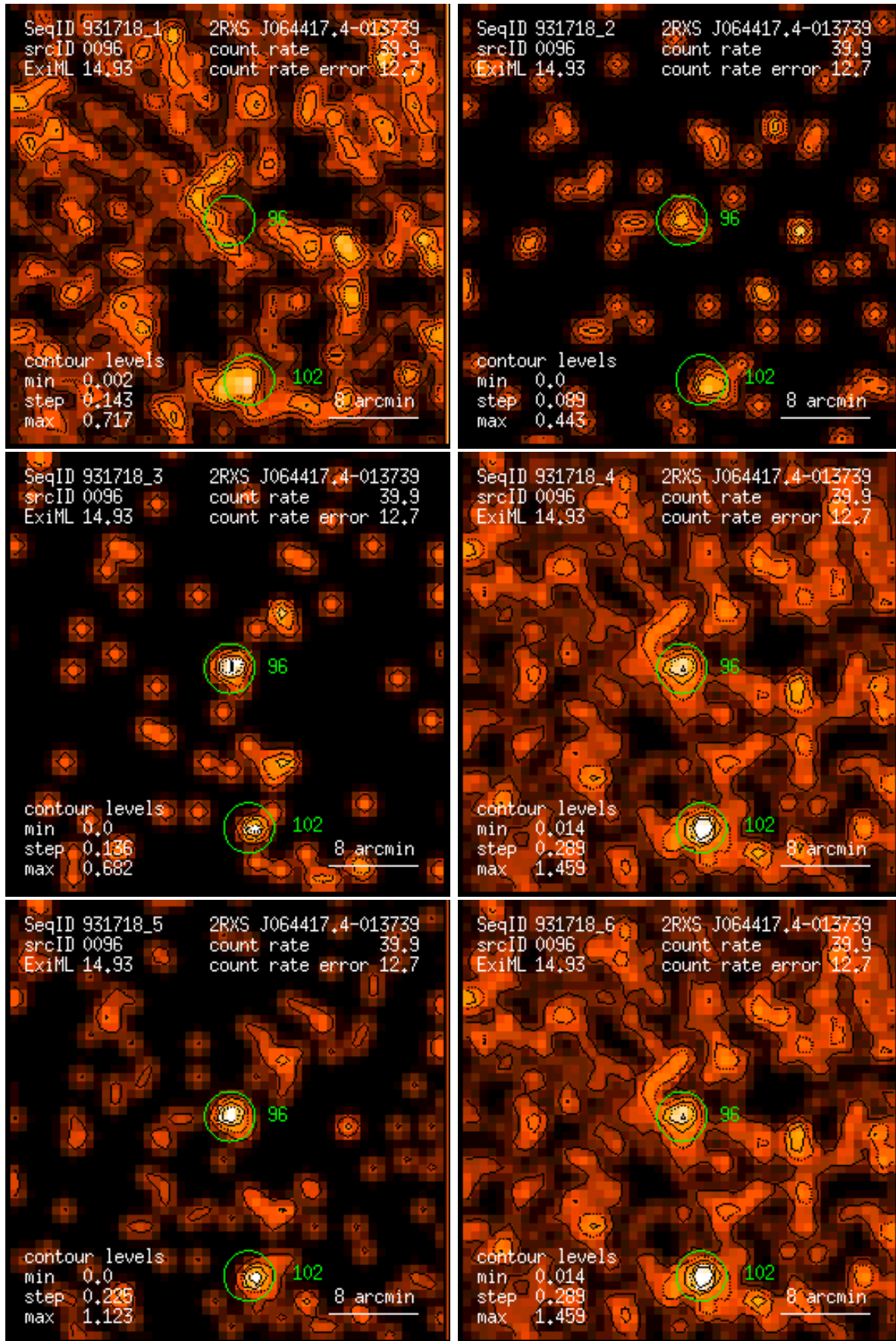
Figure 96: RASS 931718: detection 0096: band rate images, Gaussian filter: (1) PSPC channels 11 – 41, (2) 52 – 90, (3) 91 – 201, (4) 11 – 235, (5) 52 – 201, (6) 11 – 201. Broad band rates in counts/ks. Band rate contour levels in counts/ks/arcmin 2 .
