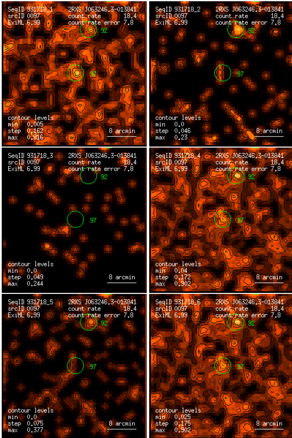
Figure 97: RASS 931718: detection 0097: band rate images, Gaussian filter: (1) PSPC channels 11 – 41, (2) 52 – 90, (3) 91 – 201, (4) 11 – 235, (5) 52 – 201, (6) 11 – 201. Broad band rates in counts/ks. Band rate contour levels in counts/ks/arcmin 2 .
