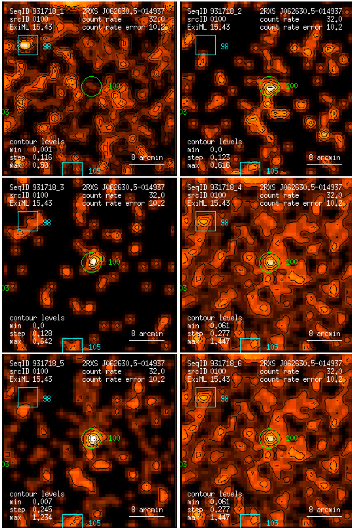
Figure 100: RASS 931718: detection 0100: band rate images, Gaussian filter: (1) PSPC channels 11 – 41, (2) 52 – 90, (3) 91 – 201, (4) 11 – 235, (5) 52 – 201, (6) 11 – 201. Broad band rates in counts/ks. Band rate contour levels in counts/ks/arcmin 2 .
