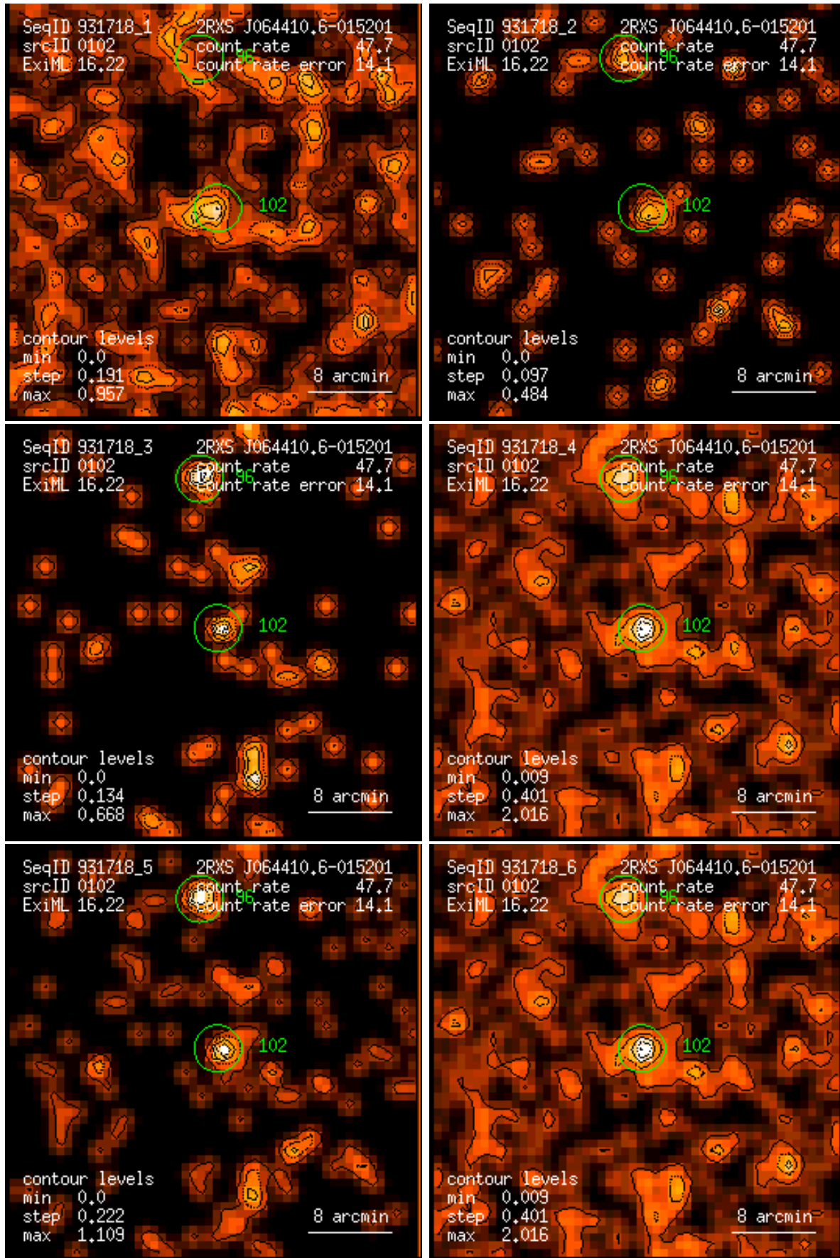
Figure 102: RASS 931718: detection 0102: band rate images, Gaussian filter: (1) PSPC channels 11 – 41, (2) 52 – 90, (3) 91 – 201, (4) 11 – 235, (5) 52 – 201, (6) 11 – 201. Broad band rates in counts/ks. Band rate contour levels in counts/ks/arcmin 2 .
