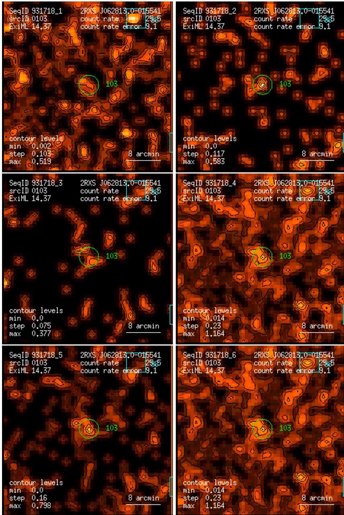
Figure 103: RASS 931718: detection 0103: band rate images, Gaussian filter: (1) PSPC channels 11 – 41, (2) 52 – 90, (3) 91 – 201, (4) 11 – 235, (5) 52 – 201, (6) 11 – 201. Broad band rates in counts/ks. Band rate contour levels in counts/ks/arcmin 2 .
