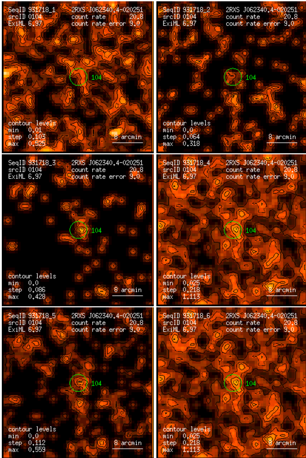
Figure 104: RASS 931718: detection 0104: band rate images, Gaussian filter: (1) PSPC channels 11 – 41, (2) 52 – 90, (3) 91 – 201, (4) 11 – 235, (5) 52 – 201, (6) 11 – 201. Broad band rates in counts/ks. Band rate contour levels in counts/ks/arcmin 2 .
