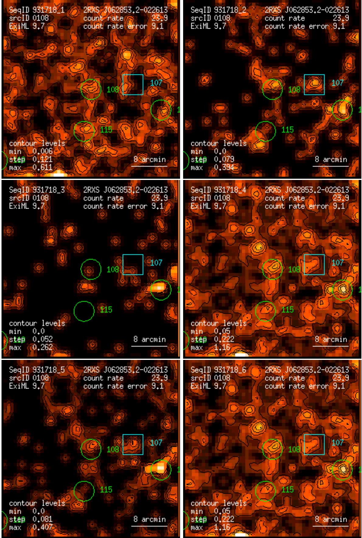
Figure 108: RASS 931718: detection 0108: band rate images, Gaussian filter: (1) PSPC channels 11 – 41, (2) 52 – 90, (3) 91 – 201, (4) 11 – 235, (5) 52 – 201, (6) 11 – 201. Broad band rates in counts/ks. Band rate contour levels in counts/ks/arcmin 2 .
