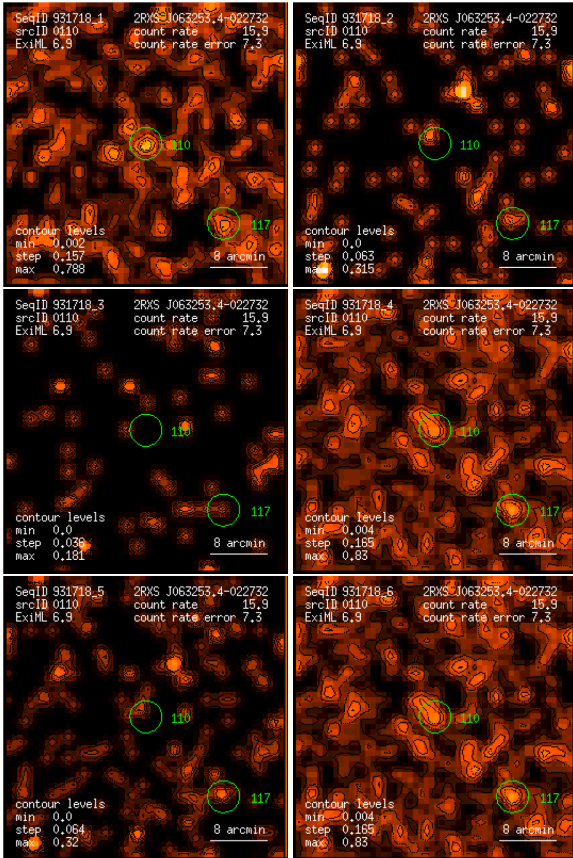
Figure 110: RASS 931718: detection 0110: band rate images, Gaussian filter: (1) PSPC channels 11 – 41, (2) 52 – 90, (3) 91 – 201, (4) 11 – 235, (5) 52 – 201, (6) 11 – 201. Broad band rates in counts/ks. Band rate contour levels in counts/ks/arcmin 2 .
