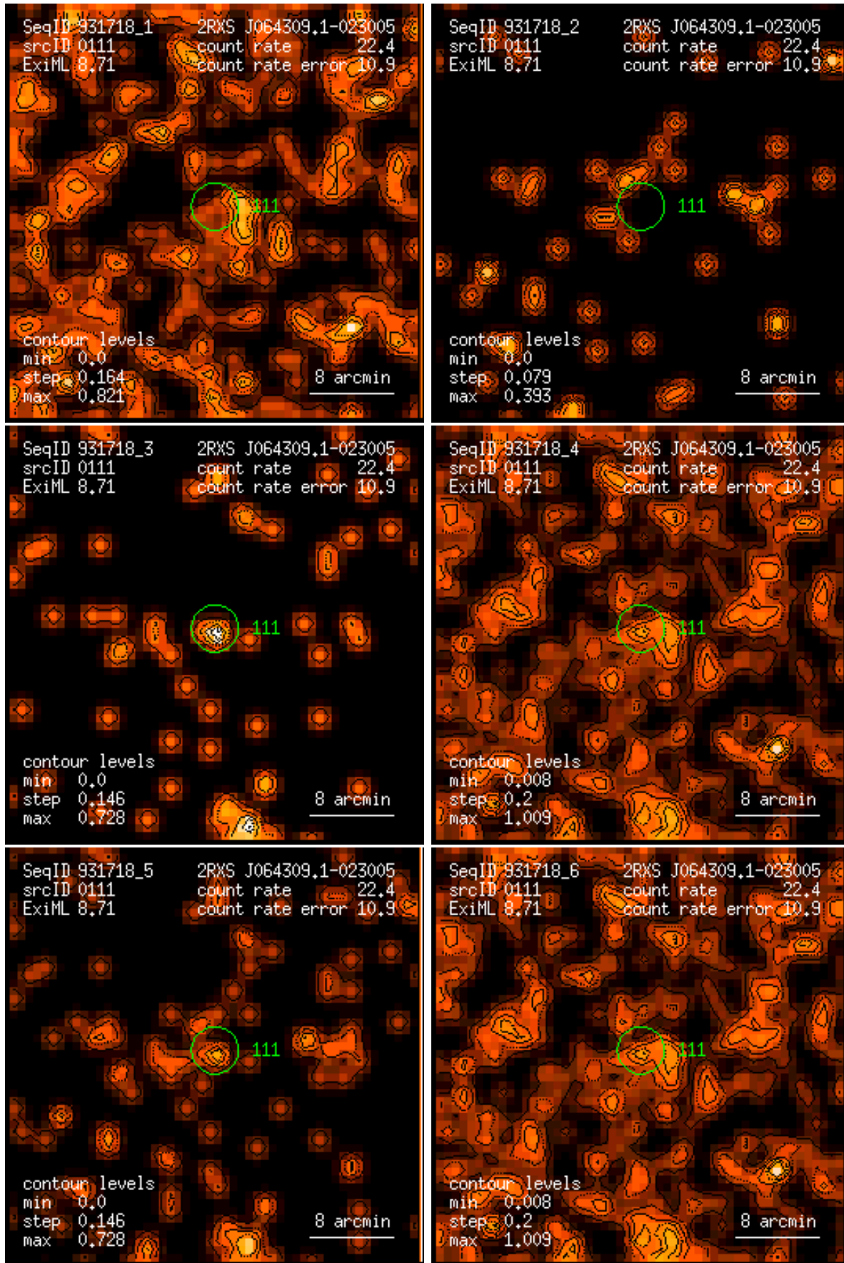
Figure 111: RASS 931718: detection 0111: band rate images, Gaussian filter: (1) PSPC channels 11 – 41, (2) 52 – 90, (3) 91 – 201, (4) 11 – 235, (5) 52 – 201, (6) 11 – 201. Broad band rates in counts/ks. Band rate contour levels in counts/ks/arcmin 2 .
