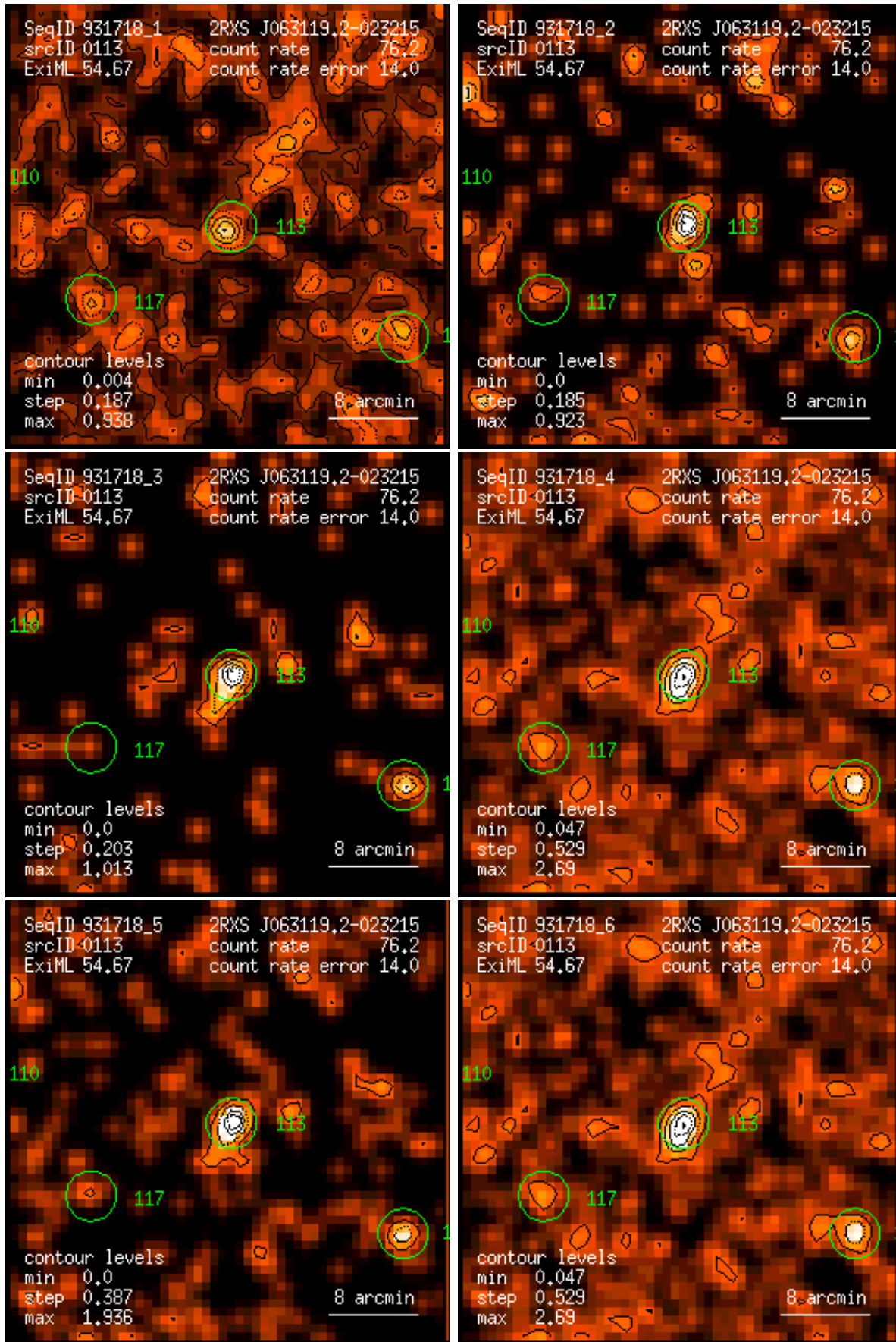
Figure 113: RASS 931718: detection 0113: band rate images, Gaussian filter: (1) PSPC channels 11 – 41, (2) 52 – 90, (3) 91 – 201, (4) 11 – 235, (5) 52 – 201, (6) 11 – 201. Broad band rates in counts/ks. Band rate contour levels in counts/ks/arcmin 2 .
