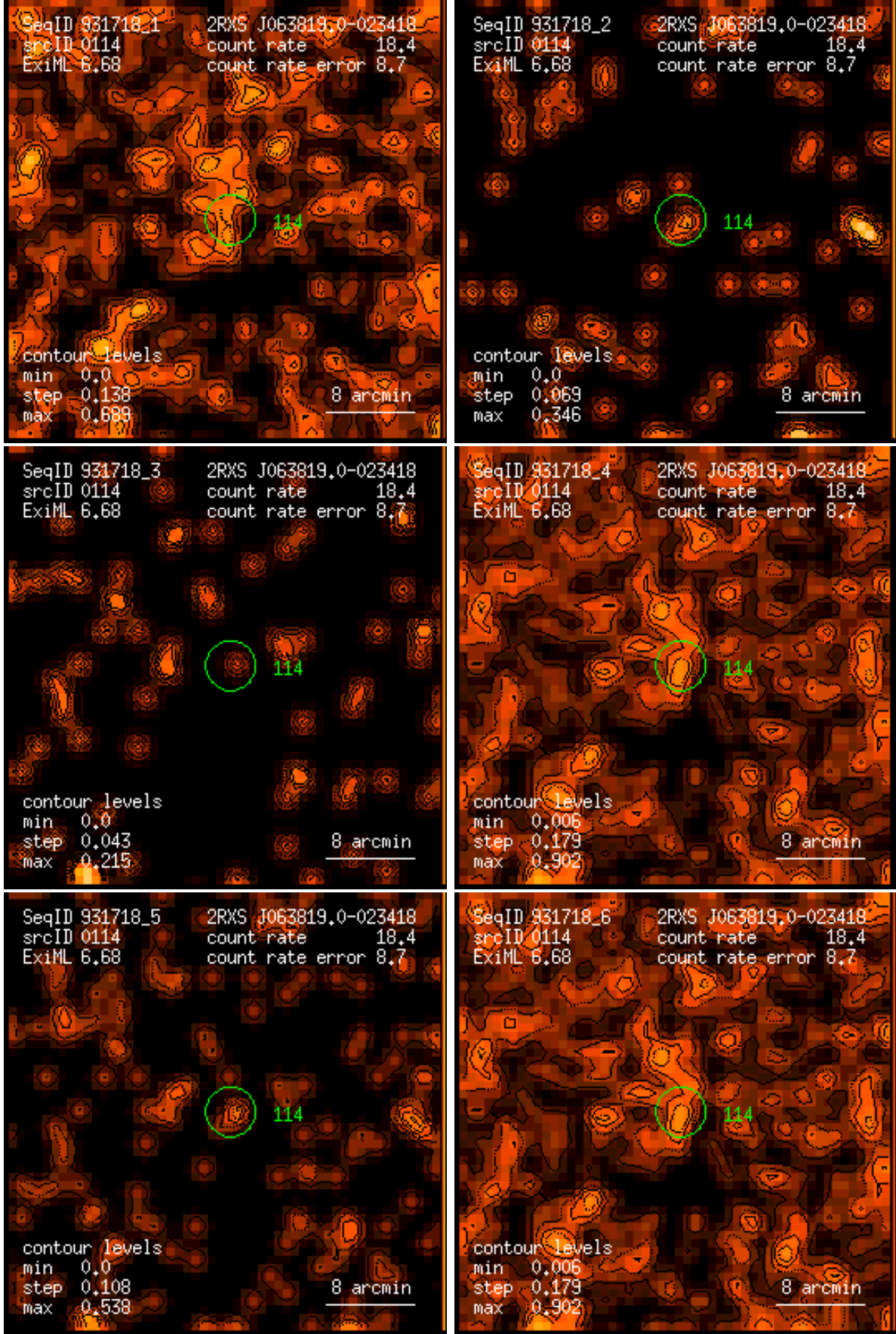
Figure 114: RASS 931718: detection 0114: band rate images, Gaussian filter: (1) PSPC channels 11 – 41, (2) 52 – 90, (3) 91 – 201, (4) 11 – 235, (5) 52 – 201, (6) 11 – 201. Broad band rates in counts/ks. Band rate contour levels in counts/ks/arcmin 2 .
