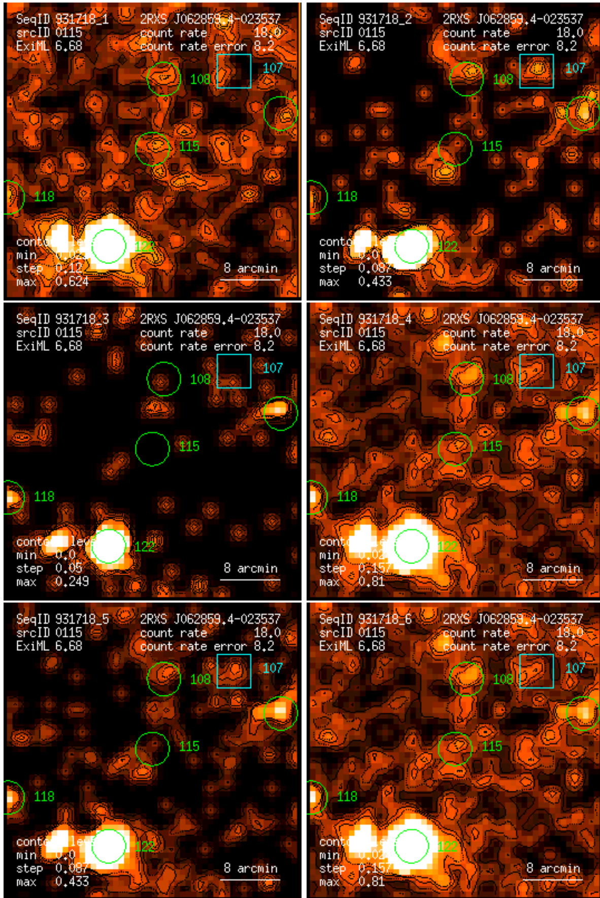
Figure 115: RASS 931718: detection 0115: band rate images, Gaussian filter: (1) PSPC channels 11 – 41, (2) 52 – 90, (3) 91 – 201, (4) 11 – 235, (5) 52 – 201, (6) 11 – 201. Broad band rates in counts/ks. Band rate contour levels in counts/ks/arcmin 2 .
