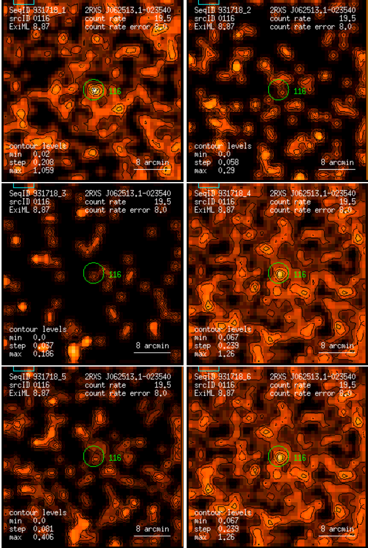
Figure 116: RASS 931718: detection 0116: band rate images, Gaussian filter: (1) PSPC channels 11 – 41, (2) 52 – 90, (3) 91 – 201, (4) 11 – 235, (5) 52 – 201, (6) 11 – 201. Broad band rates in counts/ks. Band rate contour levels in counts/ks/arcmin 2 .
