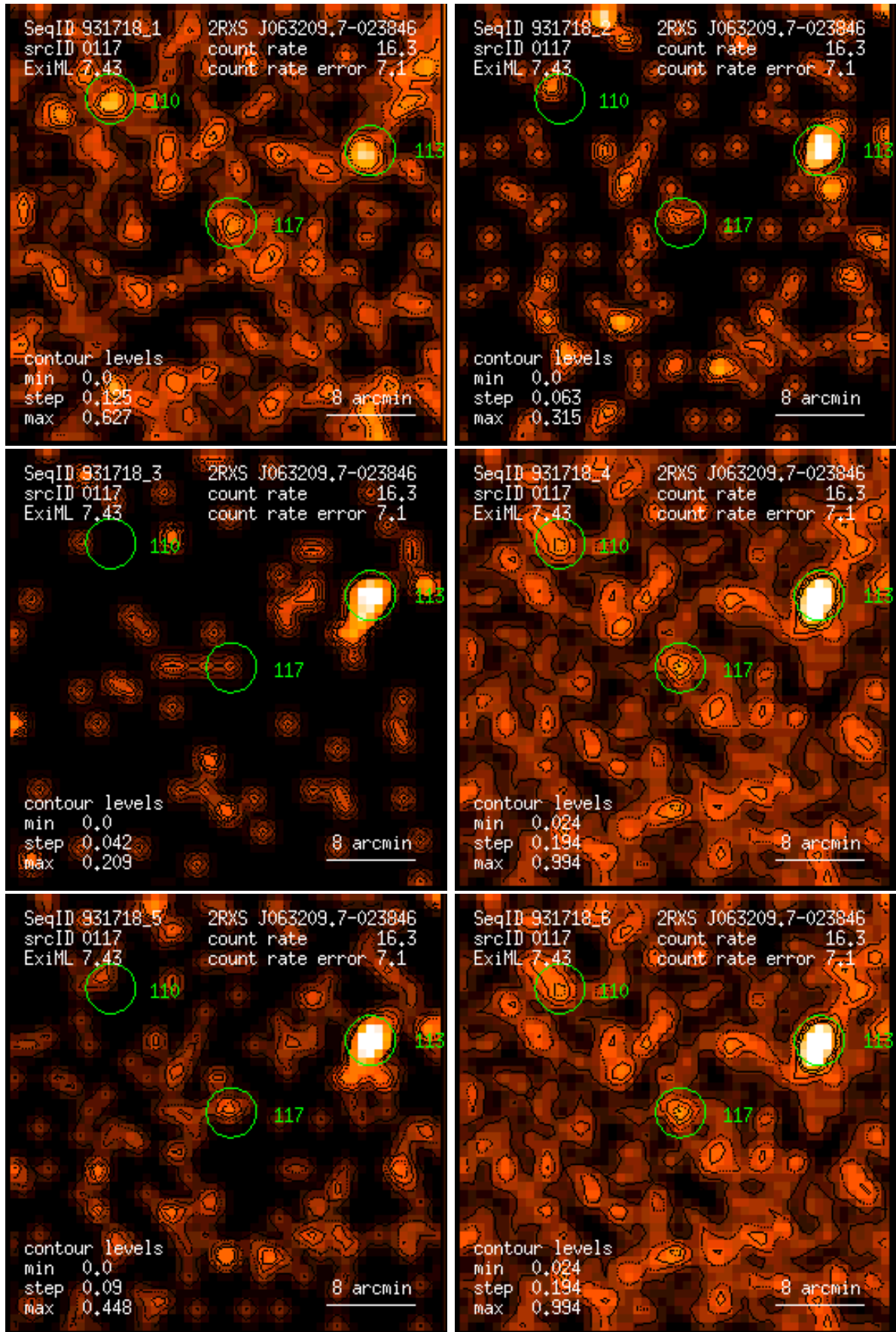
Figure 117: RASS 931718: detection 0117: band rate images, Gaussian filter: (1) PSPC channels 11 – 41, (2) 52 – 90, (3) 91 – 201, (4) 11 – 235, (5) 52 – 201, (6) 11 – 201. Broad band rates in counts/ks. Band rate contour levels in counts/ks/arcmin 2 .
