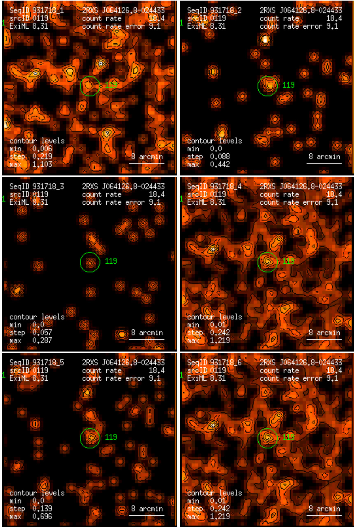
Figure 119: RASS 931718: detection 0119: band rate images, Gaussian filter: (1) PSPC channels 11 – 41, (2) 52 – 90, (3) 91 – 201, (4) 11 – 235, (5) 52 – 201, (6) 11 – 201. Broad band rates in counts/ks. Band rate contour levels in counts/ks/arcmin 2 .
