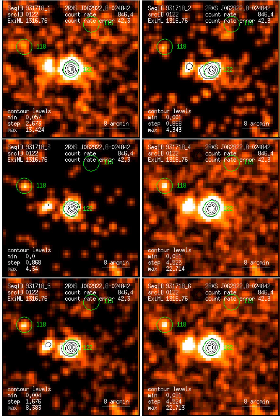
Figure 122: RASS 931718: detection 0122: band rate images, Gaussian filter: (1) PSPC channels 11 – 41, (2) 52 – 90, (3) 91 – 201, (4) 11 – 235, (5) 52 – 201, (6) 11 – 201. Broad band rates in counts/ks. Band rate contour levels in counts/ks/arcmin 2 .
