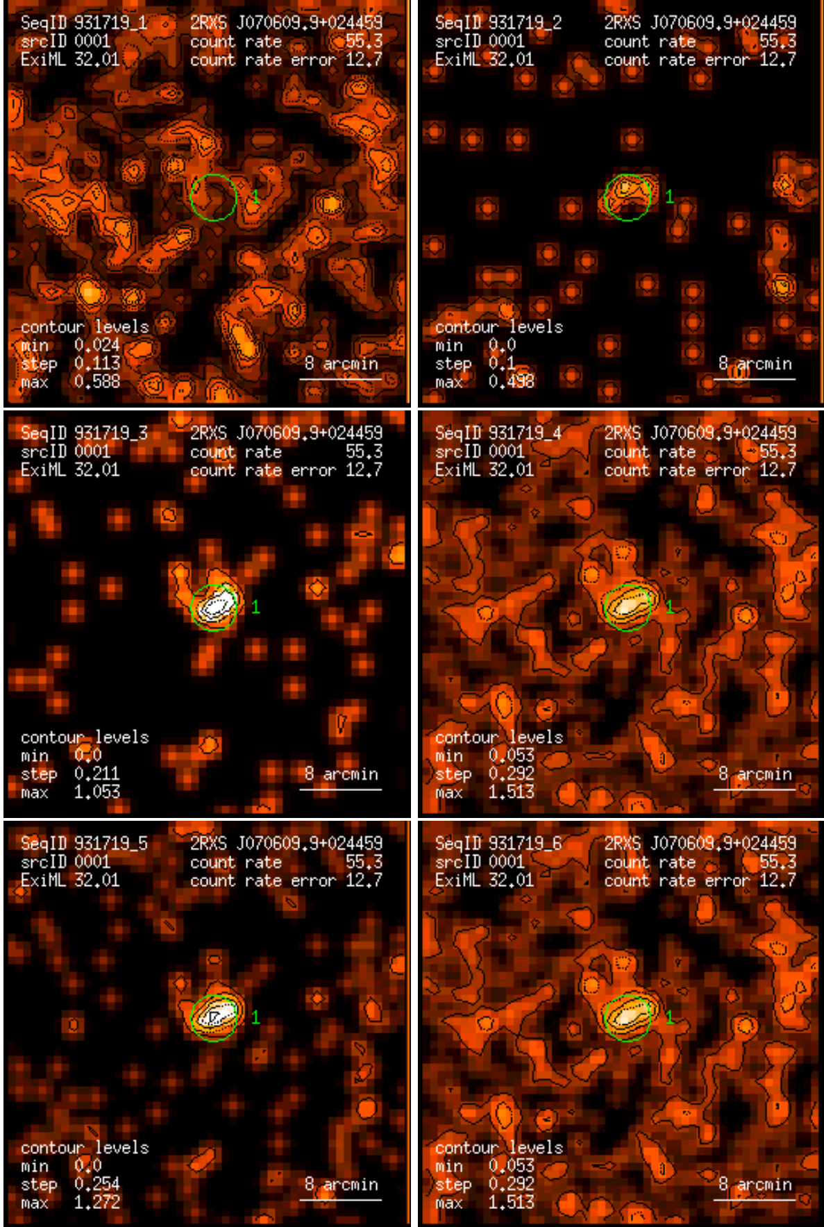
Figure 1: RASS 931719: detection 0001: band rate images, Gaussian filter: (1) PSPC channels 11 – 41, (2) 52 – 90, (3) 91 – 201, (4) 11 – 235, (5) 52 – 201, (6) 11 – 201. Broad band rates in counts/ks. Band rate contour levels in counts/ks/arcmin 2 .
