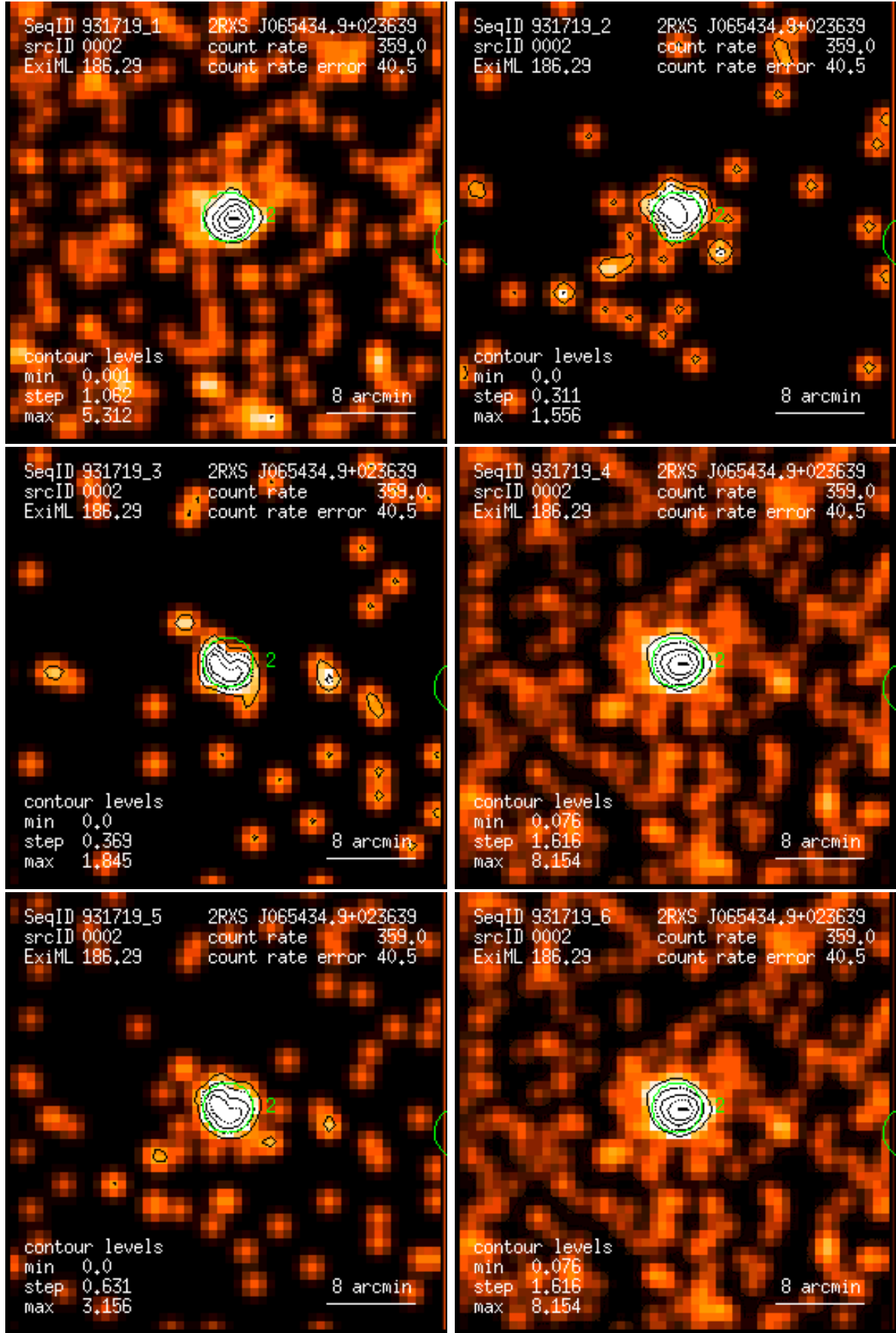
Figure 2: RASS 931719: detection 0002: band rate images, Gaussian filter: (1) PSPC channels 11 – 41, (2) 52 – 90, (3) 91 – 201, (4) 11 – 235, (5) 52 – 201, (6) 11 – 201. Broad band rates in counts/ks. Band rate contour levels in counts/ks/arcmin 2 .
