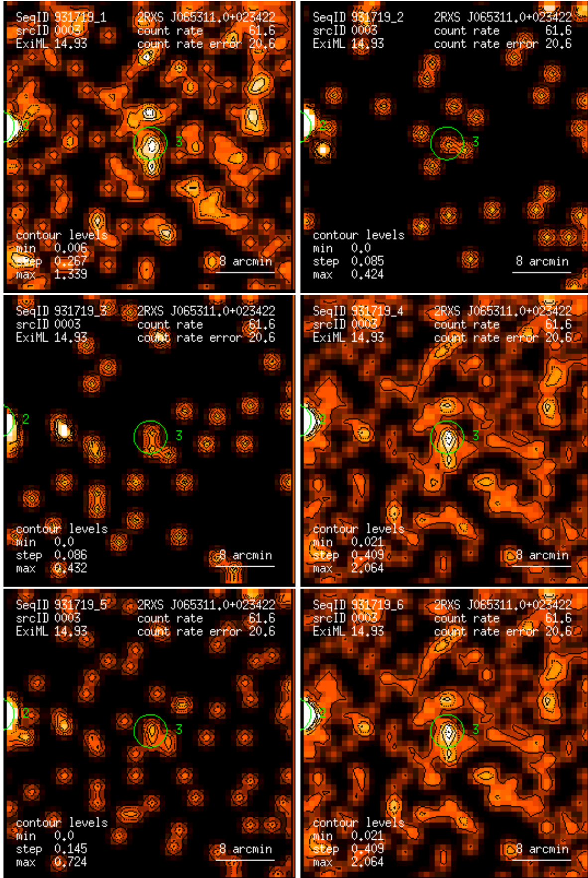
Figure 3: RASS 931719: detection 0003: band rate images, Gaussian filter: (1) PSPC channels 11 – 41, (2) 52 – 90, (3) 91 – 201, (4) 11 – 235, (5) 52 – 201, (6) 11 – 201. Broad band rates in counts/ks. Band rate contour levels in counts/ks/arcmin 2 .
