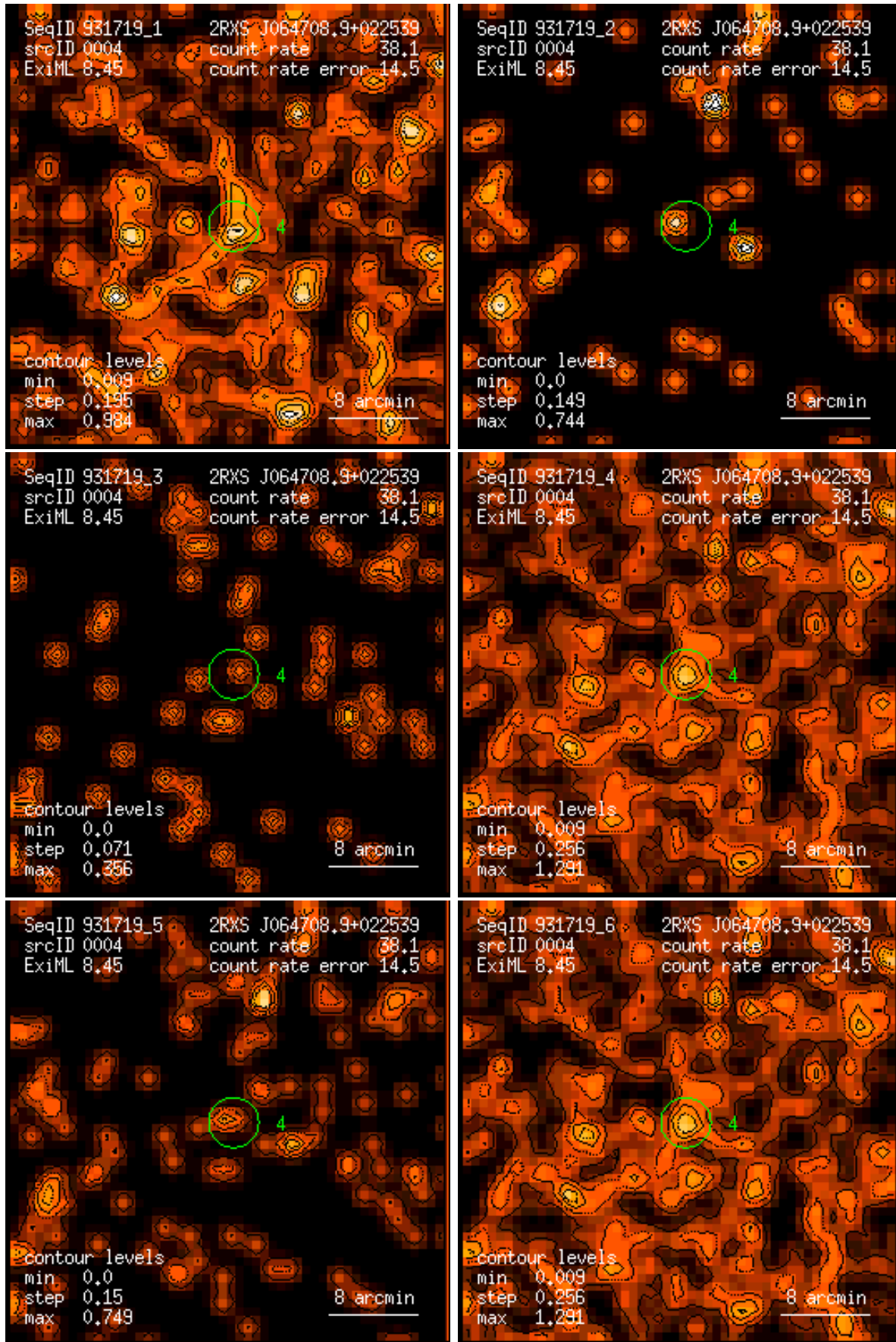
Figure 4: RASS 931719: detection 0004: band rate images, Gaussian filter: (1) PSPC channels 11 – 41, (2) 52 – 90, (3) 91 – 201, (4) 11 – 235, (5) 52 – 201, (6) 11 – 201. Broad band rates in counts/ks. Band rate contour levels in counts/ks/arcmin 2 .
