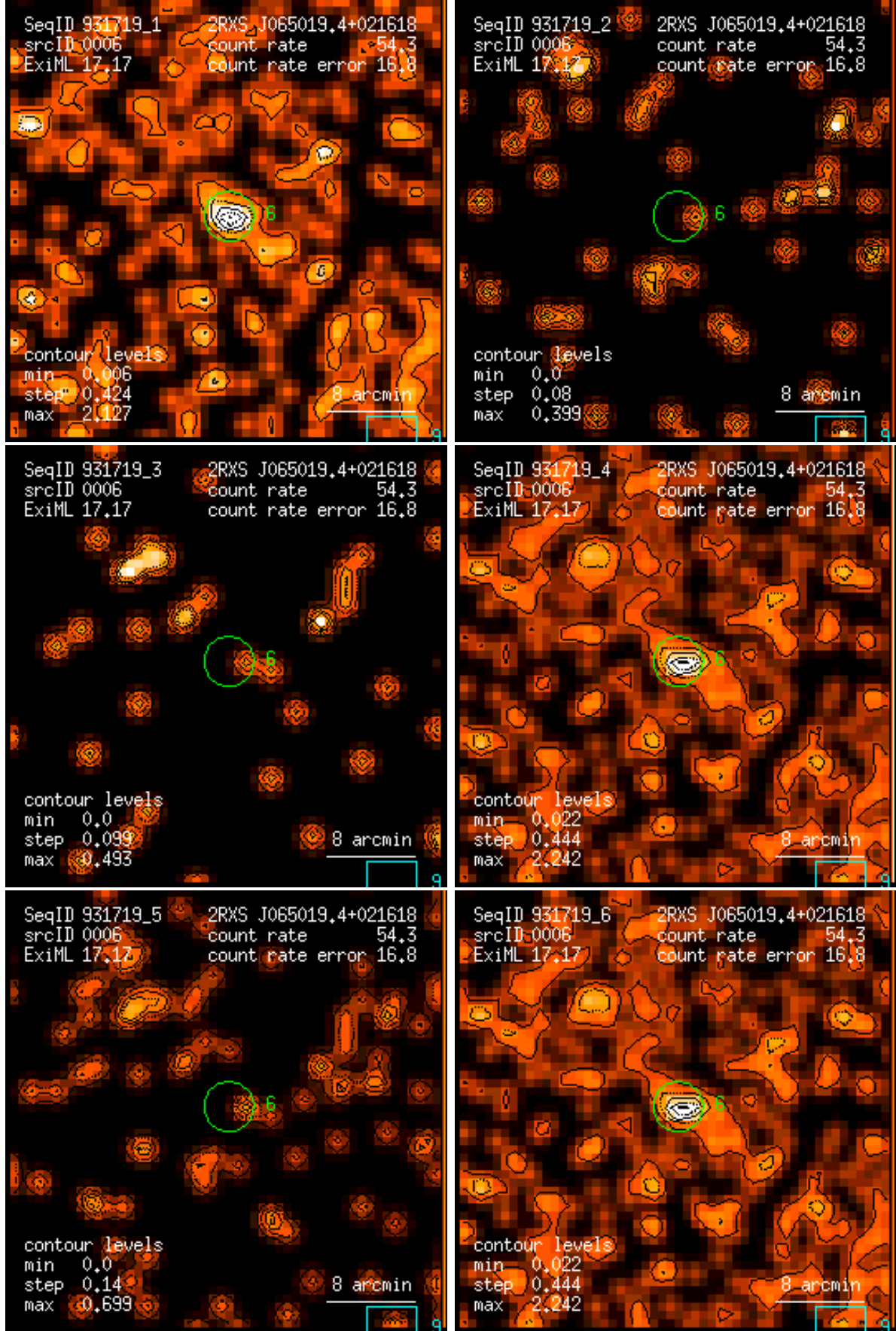
Figure 6: RASS 931719: detection 0006: band rate images, Gaussian filter: (1) PSPC channels 11 – 41, (2) 52 – 90, (3) 91 – 201, (4) 11 – 235, (5) 52 – 201, (6) 11 – 201. Broad band rates in counts/ks. Band rate contour levels in counts/ks/arcmin 2 .
