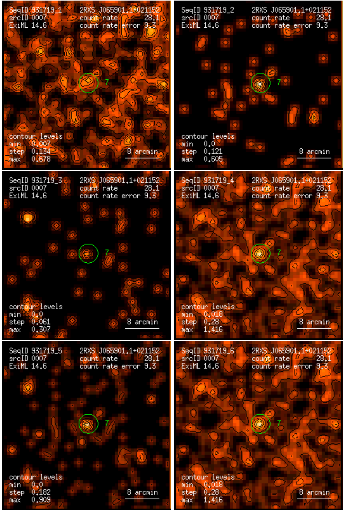
Figure 7: RASS 931719: detection 0007: band rate images, Gaussian filter: (1) PSPC channels 11 – 41, (2) 52 – 90, (3) 91 – 201, (4) 11 – 235, (5) 52 – 201, (6) 11 – 201. Broad band rates in counts/ks. Band rate contour levels in counts/ks/arcmin 2 .
