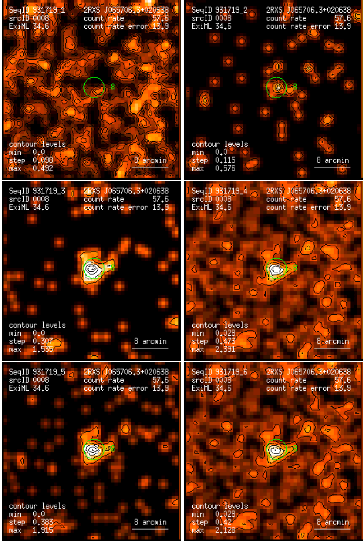
Figure 8: RASS 931719: detection 0008: band rate images, Gaussian filter: (1) PSPC channels 11 – 41, (2) 52 – 90, (3) 91 – 201, (4) 11 – 235, (5) 52 – 201, (6) 11 – 201. Broad band rates in counts/ks. Band rate contour levels in counts/ks/arcmin 2 .
