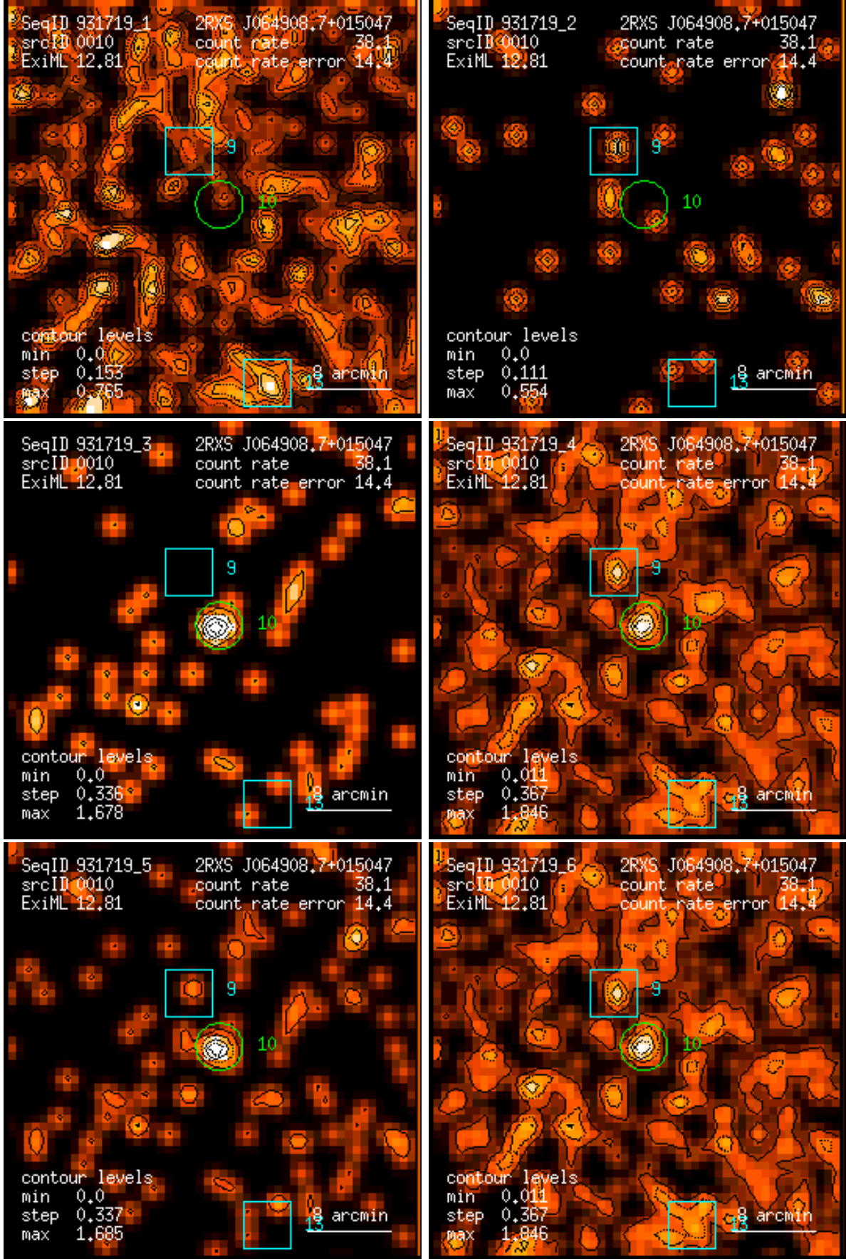
Figure 10: RASS 931719: detection 0010: band rate images, Gaussian filter: (1) PSPC channels 11 – 41, (2) 52 – 90, (3) 91 – 201, (4) 11 – 235, (5) 52 – 201, (6) 11 – 201. Broad band rates in counts/ks. Band rate contour levels in counts/ks/arcmin 2 .
