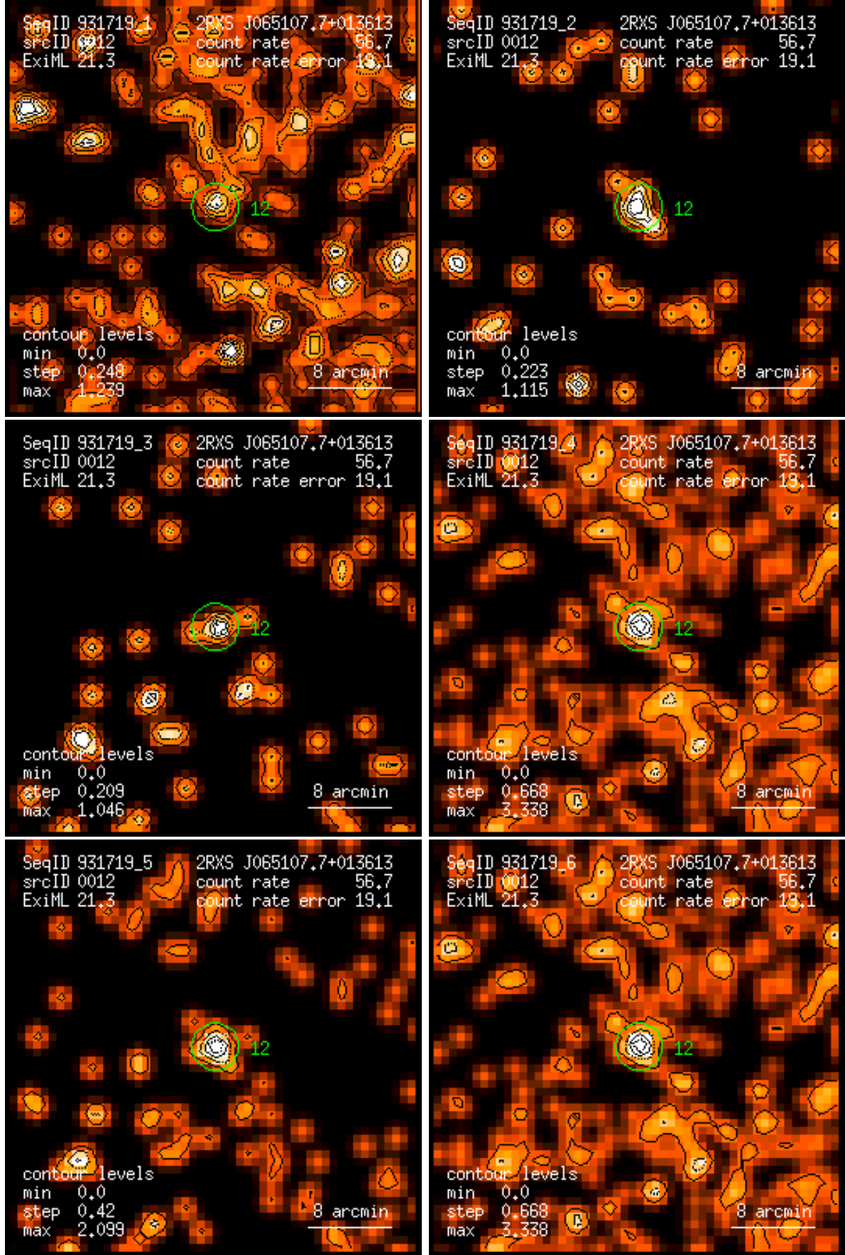
Figure 12: RASS 931719: detection 0012: band rate images, Gaussian filter: (1) PSPC channels 11 – 41, (2) 52 – 90, (3) 91 – 201, (4) 11 – 235, (5) 52 – 201, (6) 11 – 201. Broad band rates in counts/ks. Band rate contour levels in counts/ks/arcmin 2 .
