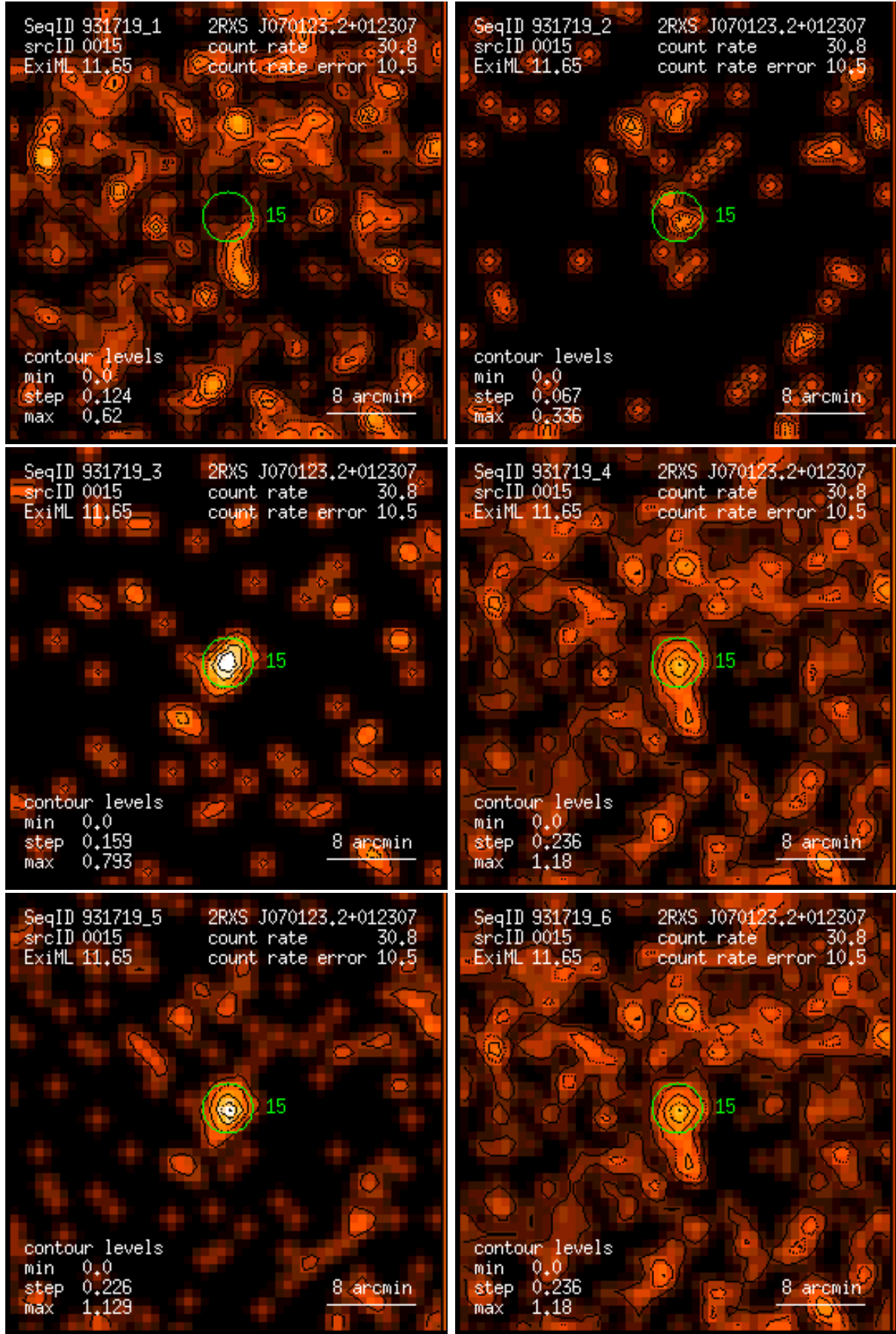
Figure 15: RASS 931719: detection 0015: band rate images, Gaussian filter: (1) PSPC channels 11 – 41, (2) 52 – 90, (3) 91 – 201, (4) 11 – 235, (5) 52 – 201, (6) 11 – 201. Broad band rates in counts/ks. Band rate contour levels in counts/ks/arcmin 2 .
