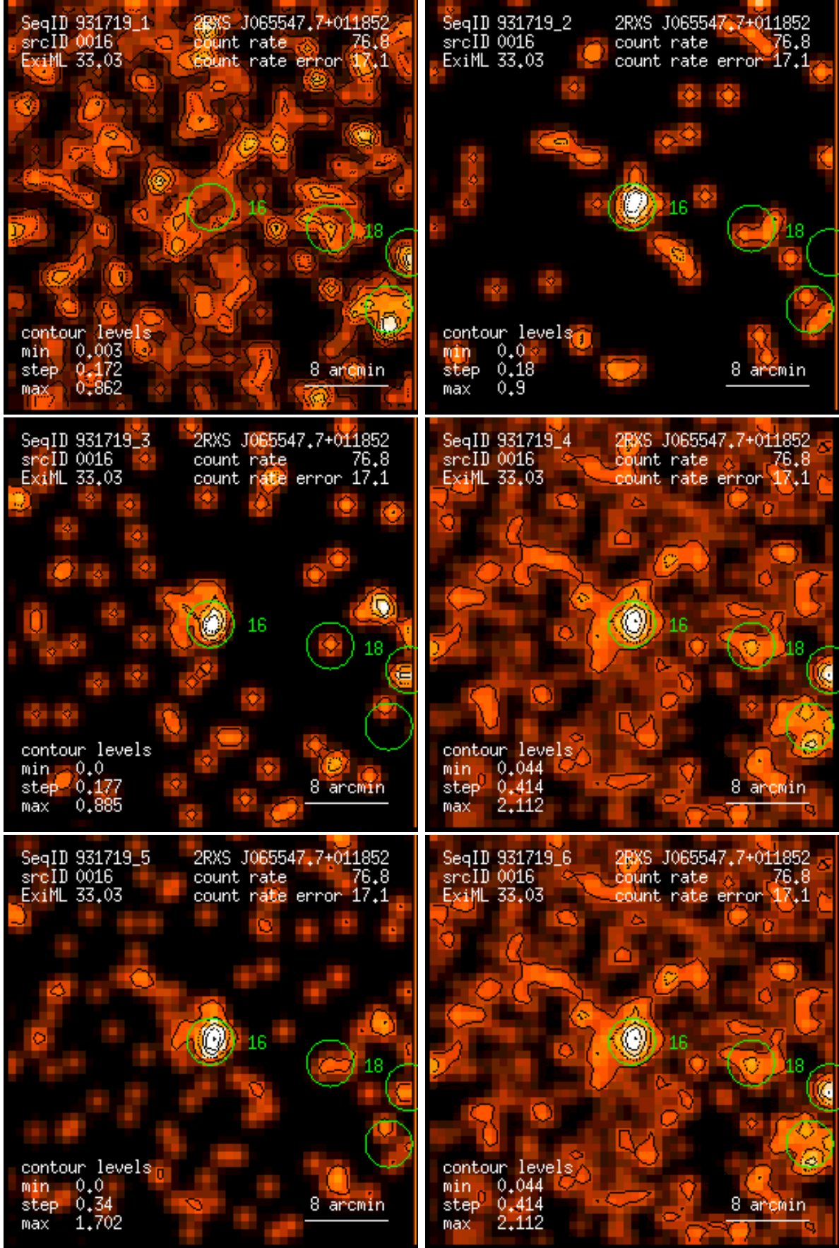
Figure 16: RASS 931719: detection 0016: band rate images, Gaussian filter: (1) PSPC channels 11 – 41, (2) 52 – 90, (3) 91 – 201, (4) 11 – 235, (5) 52 – 201, (6) 11 – 201. Broad band rates in counts/ks. Band rate contour levels in counts/ks/arcmin 2 .
