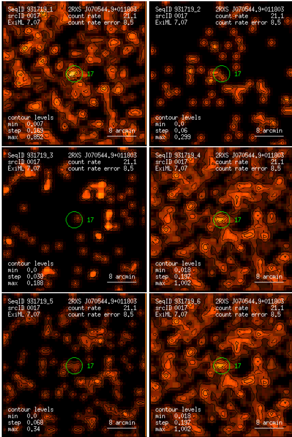
Figure 17: RASS 931719: detection 0017: band rate images, Gaussian filter: (1) PSPC channels 11 – 41, (2) 52 – 90, (3) 91 – 201, (4) 11 – 235, (5) 52 – 201, (6) 11 – 201. Broad band rates in counts/ks. Band rate contour levels in counts/ks/arcmin 2 .
