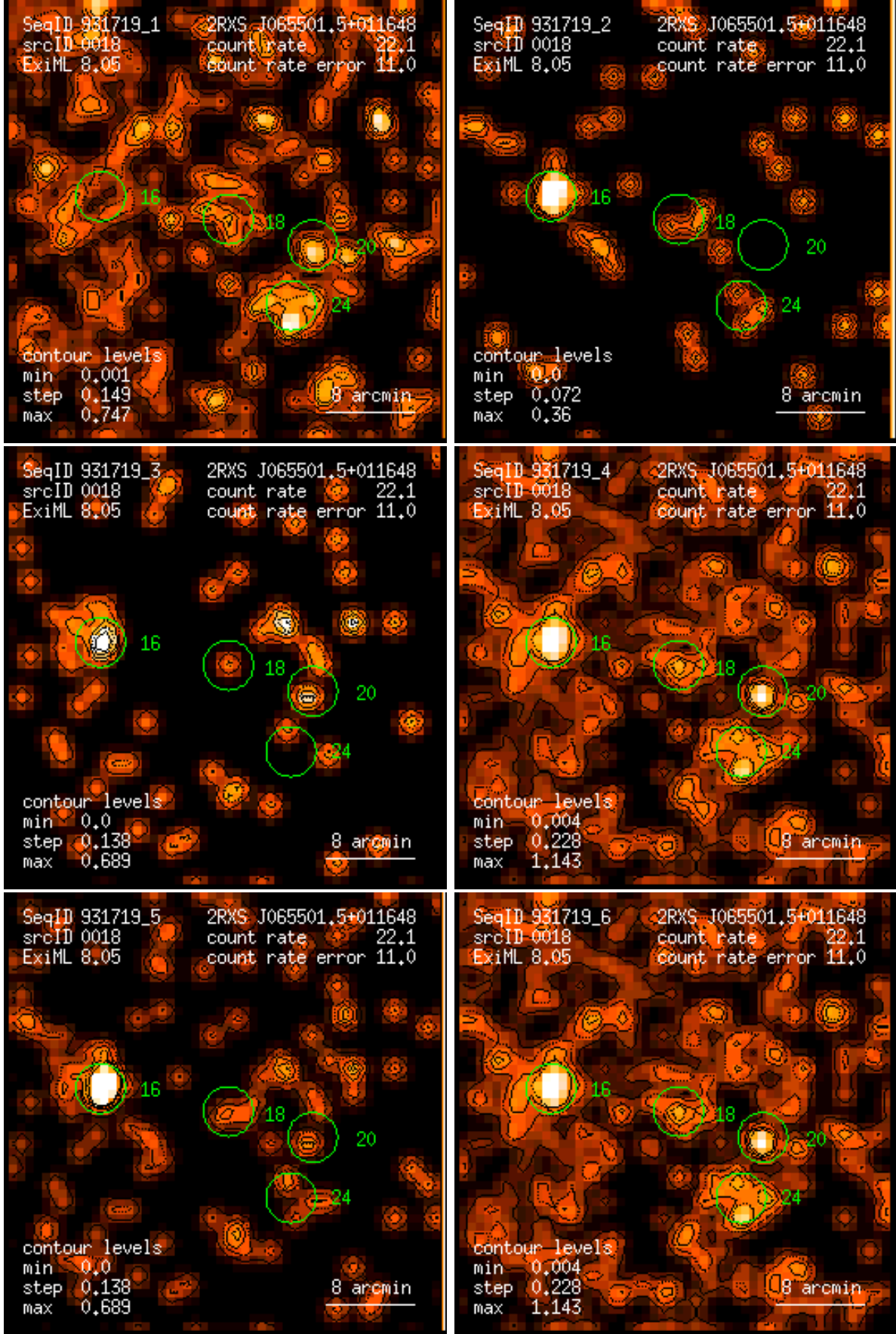
Figure 18: RASS 931719: detection 0018: band rate images, Gaussian filter: (1) PSPC channels 11 – 41, (2) 52 – 90, (3) 91 – 201, (4) 11 – 235, (5) 52 – 201, (6) 11 – 201. Broad band rates in counts/ks. Band rate contour levels in counts/ks/arcmin 2 .
