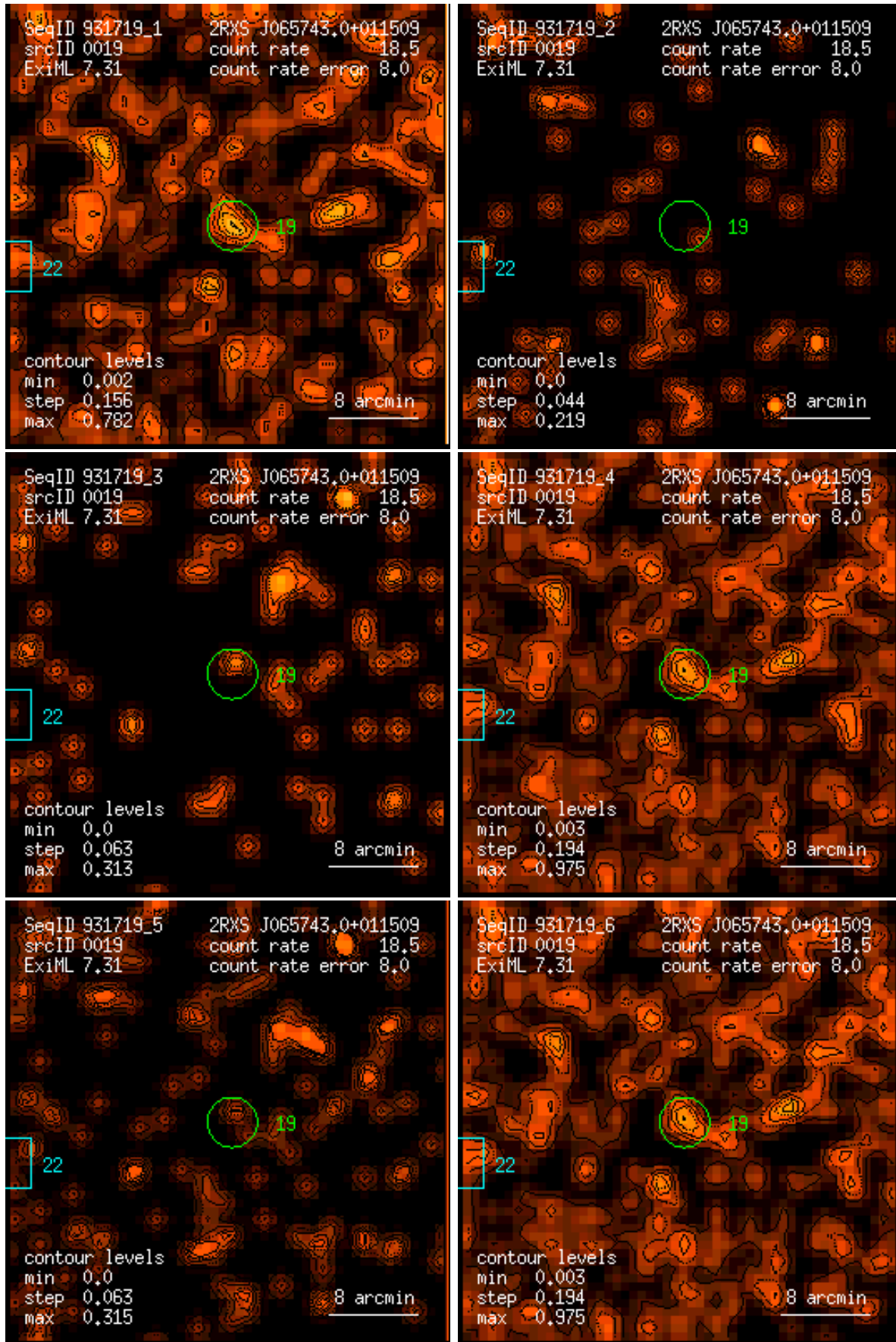
Figure 19: RASS 931719: detection 0019: band rate images, Gaussian filter: (1) PSPC channels 11 – 41, (2) 52 – 90, (3) 91 – 201, (4) 11 – 235, (5) 52 – 201, (6) 11 – 201. Broad band rates in counts/ks. Band rate contour levels in counts/ks/arcmin 2 .
