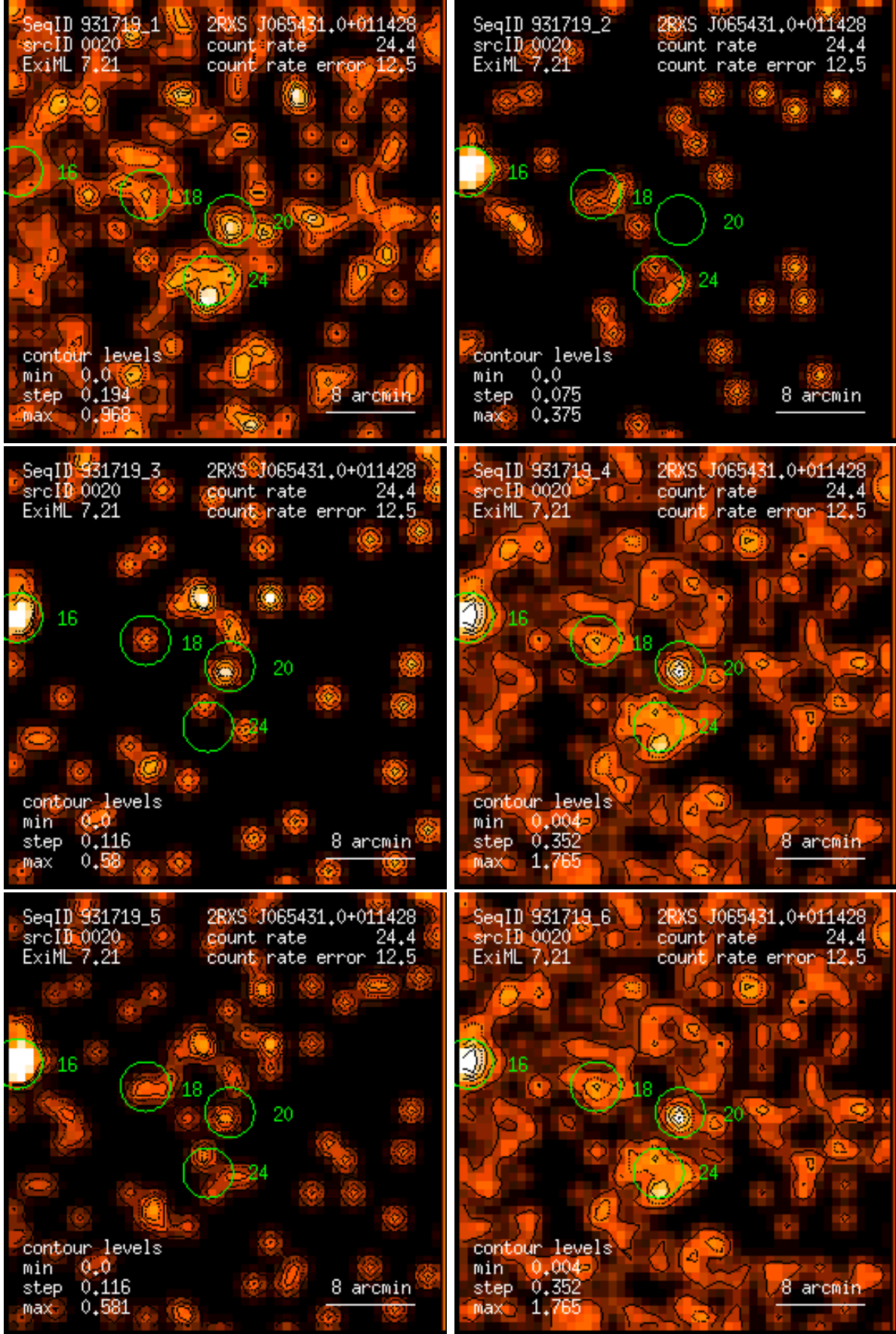
Figure 20: RASS 931719: detection 0020: band rate images, Gaussian filter: (1) PSPC channels 11 – 41, (2) 52 – 90, (3) 91 – 201, (4) 11 – 235, (5) 52 – 201, (6) 11 – 201. Broad band rates in counts/ks. Band rate contour levels in counts/ks/arcmin 2 .
