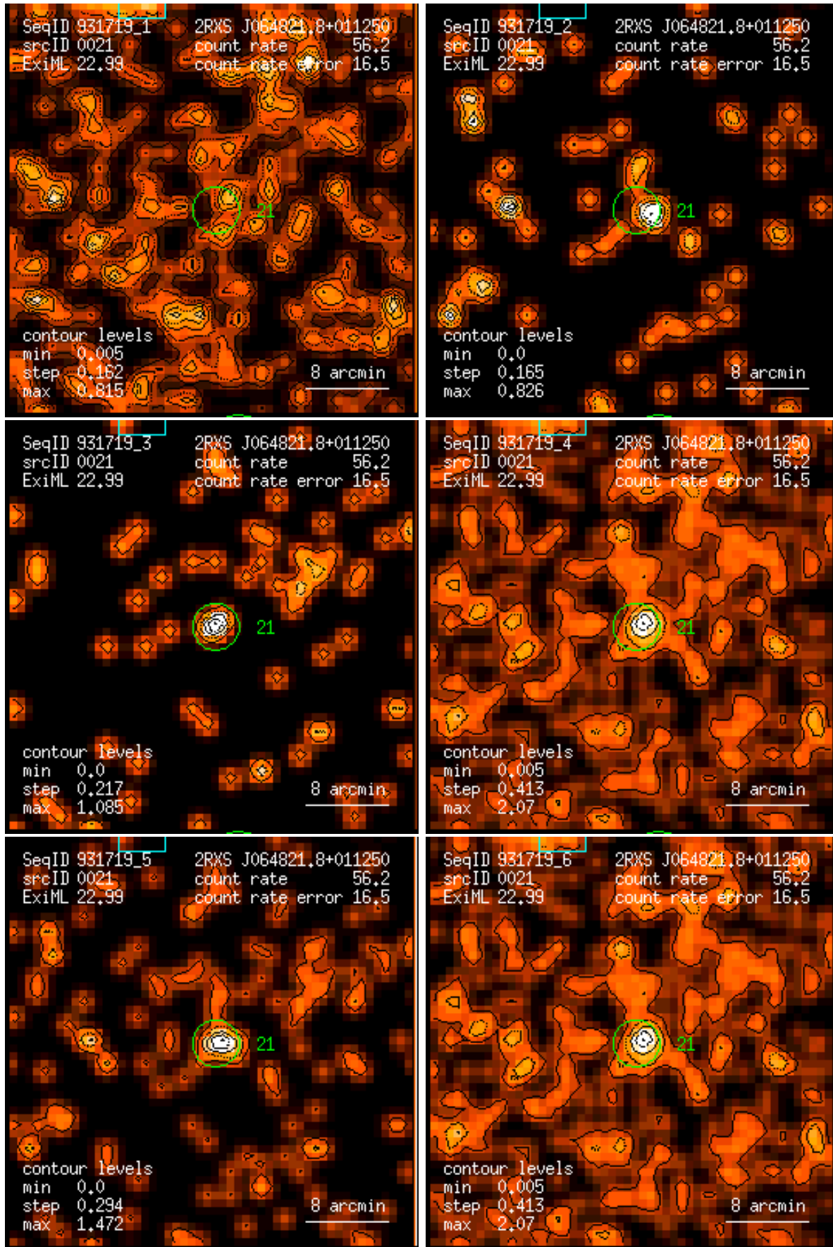
Figure 21: RASS 931719: detection 0021: band rate images, Gaussian filter: (1) PSPC channels 11 – 41, (2) 52 – 90, (3) 91 – 201, (4) 11 – 235, (5) 52 – 201, (6) 11 – 201. Broad band rates in counts/ks. Band rate contour levels in counts/ks/arcmin 2 .
