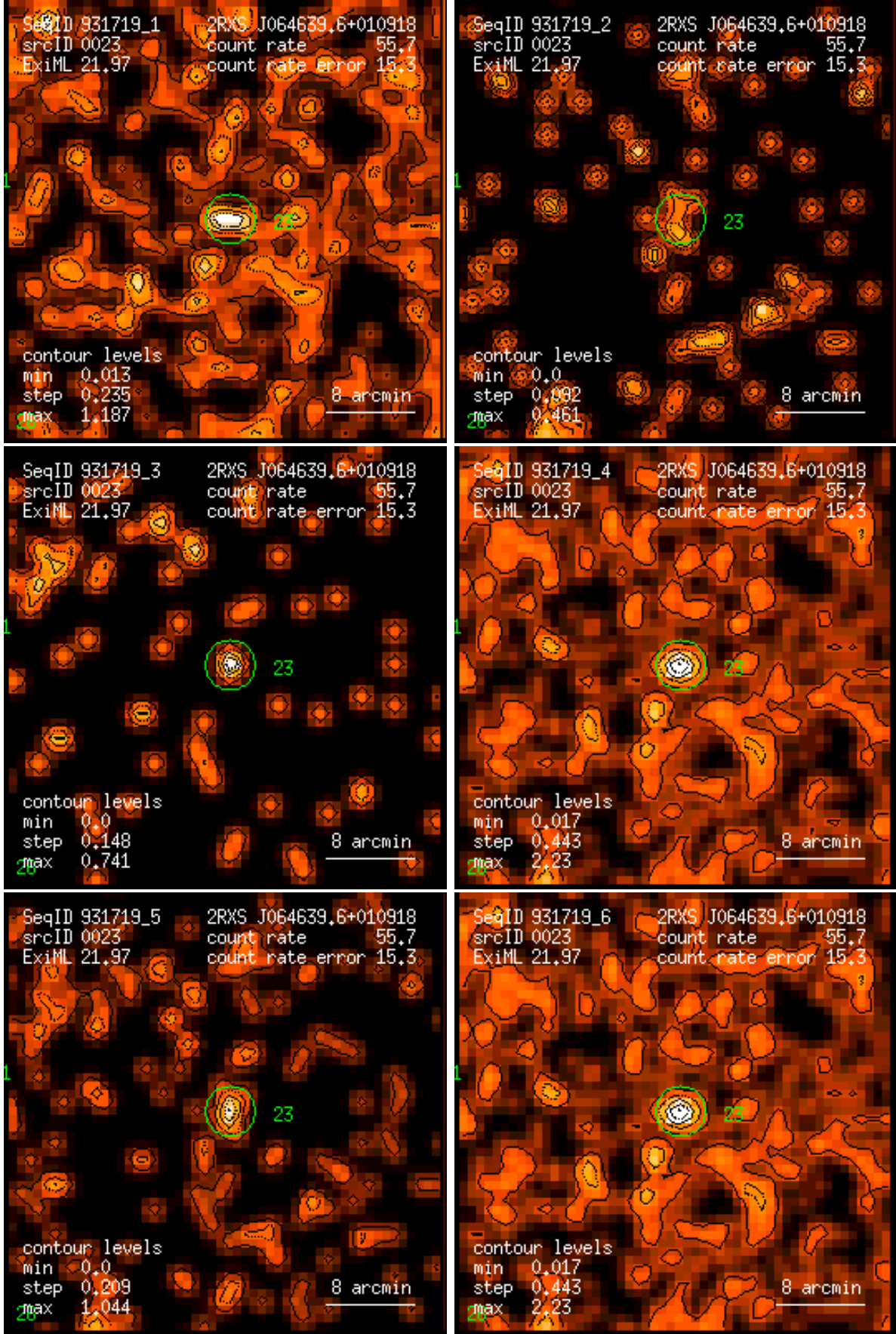
Figure 23: RASS 931719: detection 0023: band rate images, Gaussian filter: (1) PSPC channels 11 – 41, (2) 52 – 90, (3) 91 – 201, (4) 11 – 235, (5) 52 – 201, (6) 11 – 201. Broad band rates in counts/ks. Band rate contour levels in counts/ks/arcmin 2 .
