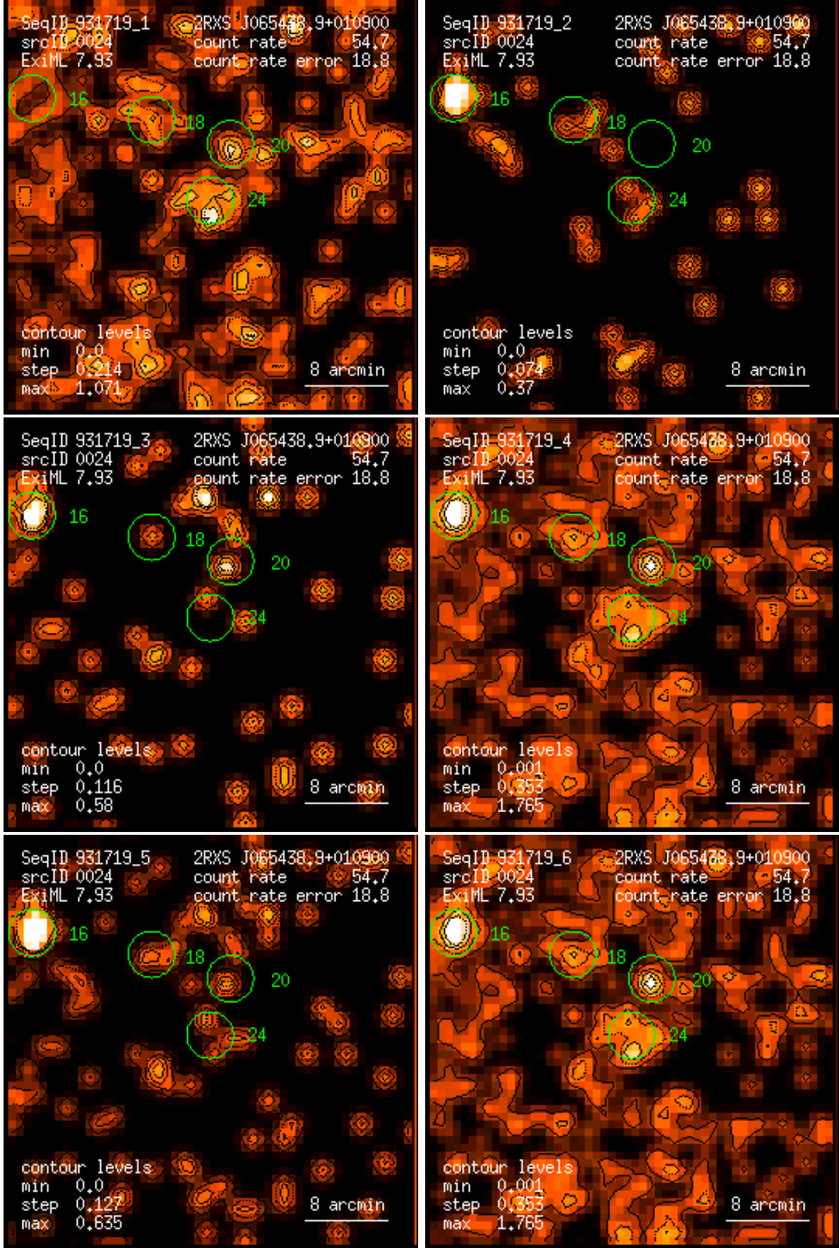
Figure 24: RASS 931719: detection 0024: band rate images, Gaussian filter: (1) PSPC channels 11 – 41, (2) 52 – 90, (3) 91 – 201, (4) 11 – 235, (5) 52 – 201, (6) 11 – 201. Broad band rates in counts/ks. Band rate contour levels in counts/ks/arcmin 2 .
