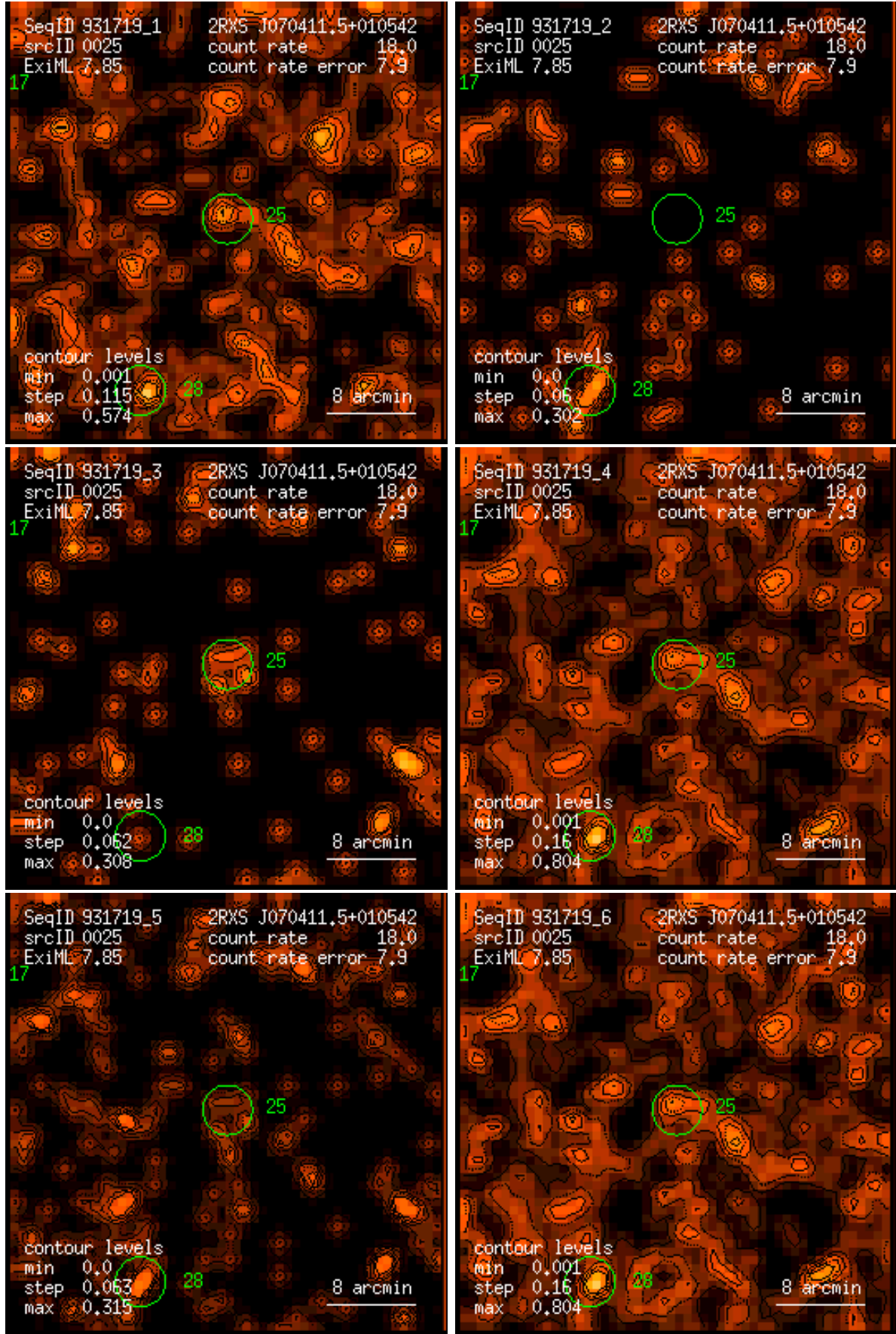
Figure 25: RASS 931719: detection 0025: band rate images, Gaussian filter: (1) PSPC channels 11 – 41, (2) 52 – 90, (3) 91 – 201, (4) 11 – 235, (5) 52 – 201, (6) 11 – 201. Broad band rates in counts/ks. Band rate contour levels in counts/ks/arcmin 2 .
