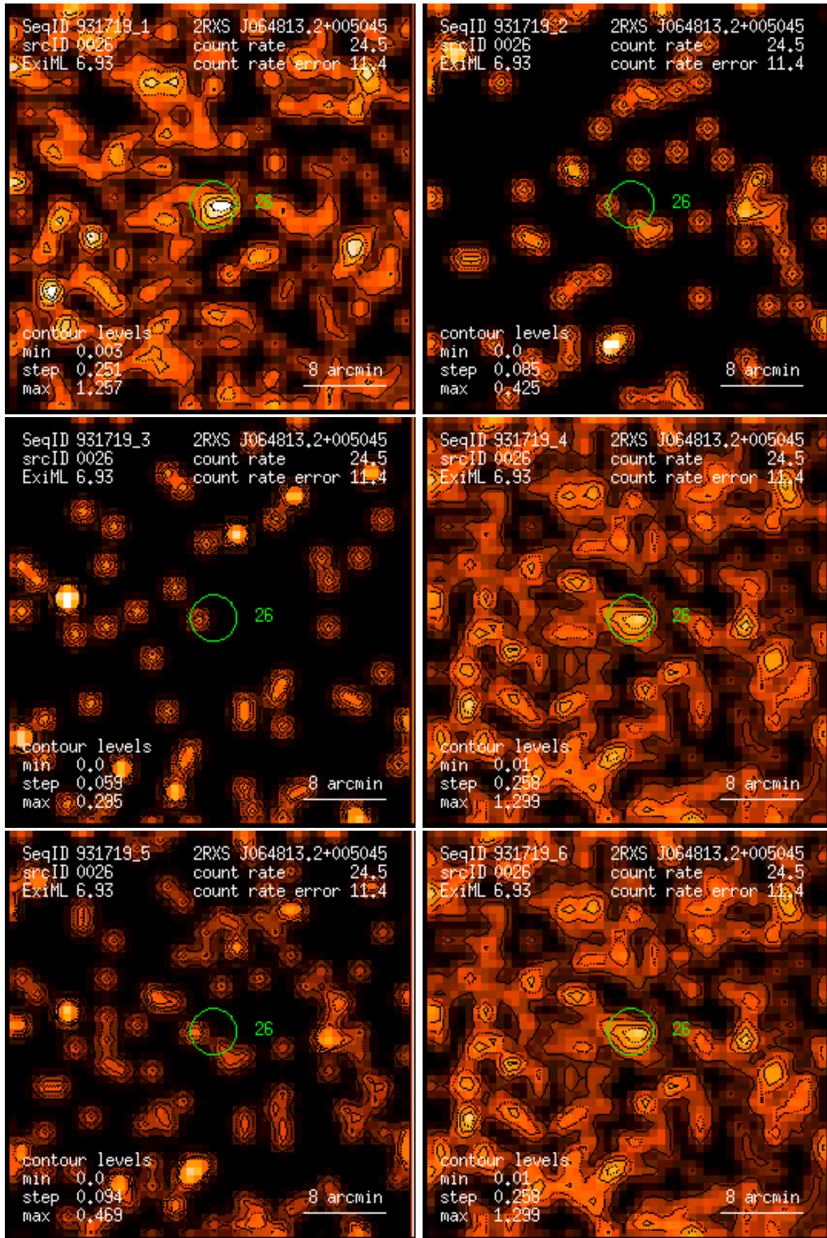
Figure 26: RASS 931719: detection 0026: band rate images, Gaussian filter: (1) PSPC channels 11 – 41, (2) 52 – 90, (3) 91 – 201, (4) 11 – 235, (5) 52 – 201, (6) 11 – 201. Broad band rates in counts/ks. Band rate contour levels in counts/ks/arcmin 2 .
