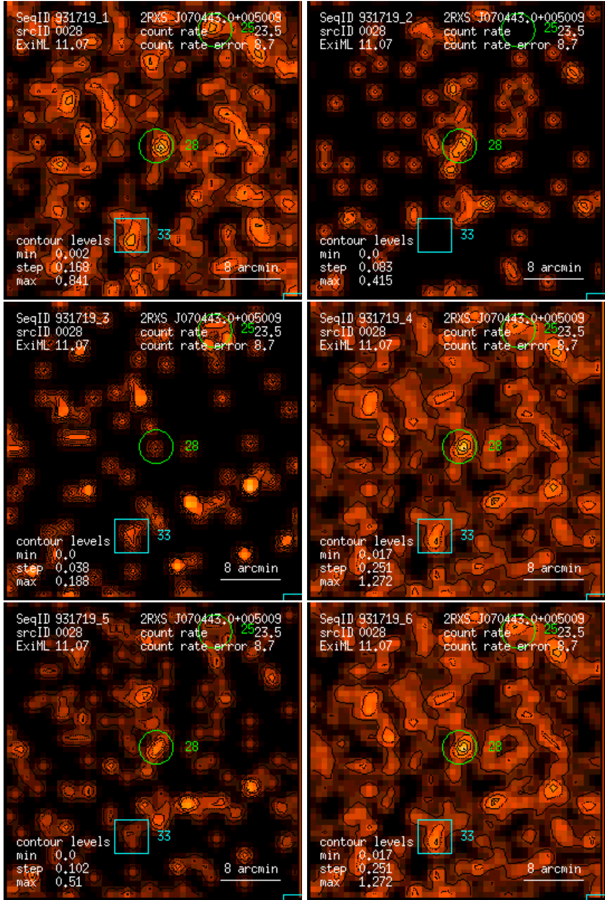
Figure 28: RASS 931719: detection 0028: band rate images, Gaussian filter: (1) PSPC channels 11 – 41, (2) 52 – 90, (3) 91 – 201, (4) 11 – 235, (5) 52 – 201, (6) 11 – 201. Broad band rates in counts/ks. Band rate contour levels in counts/ks/arcmin 2 .
