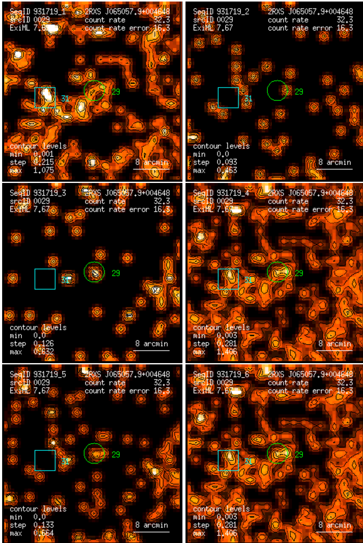
Figure 29: RASS 931719: detection 0029: band rate images, Gaussian filter: (1) PSPC channels 11 – 41, (2) 52 – 90, (3) 91 – 201, (4) 11 – 235, (5) 52 – 201, (6) 11 – 201. Broad band rates in counts/ks. Band rate contour levels in counts/ks/arcmin 2 .
