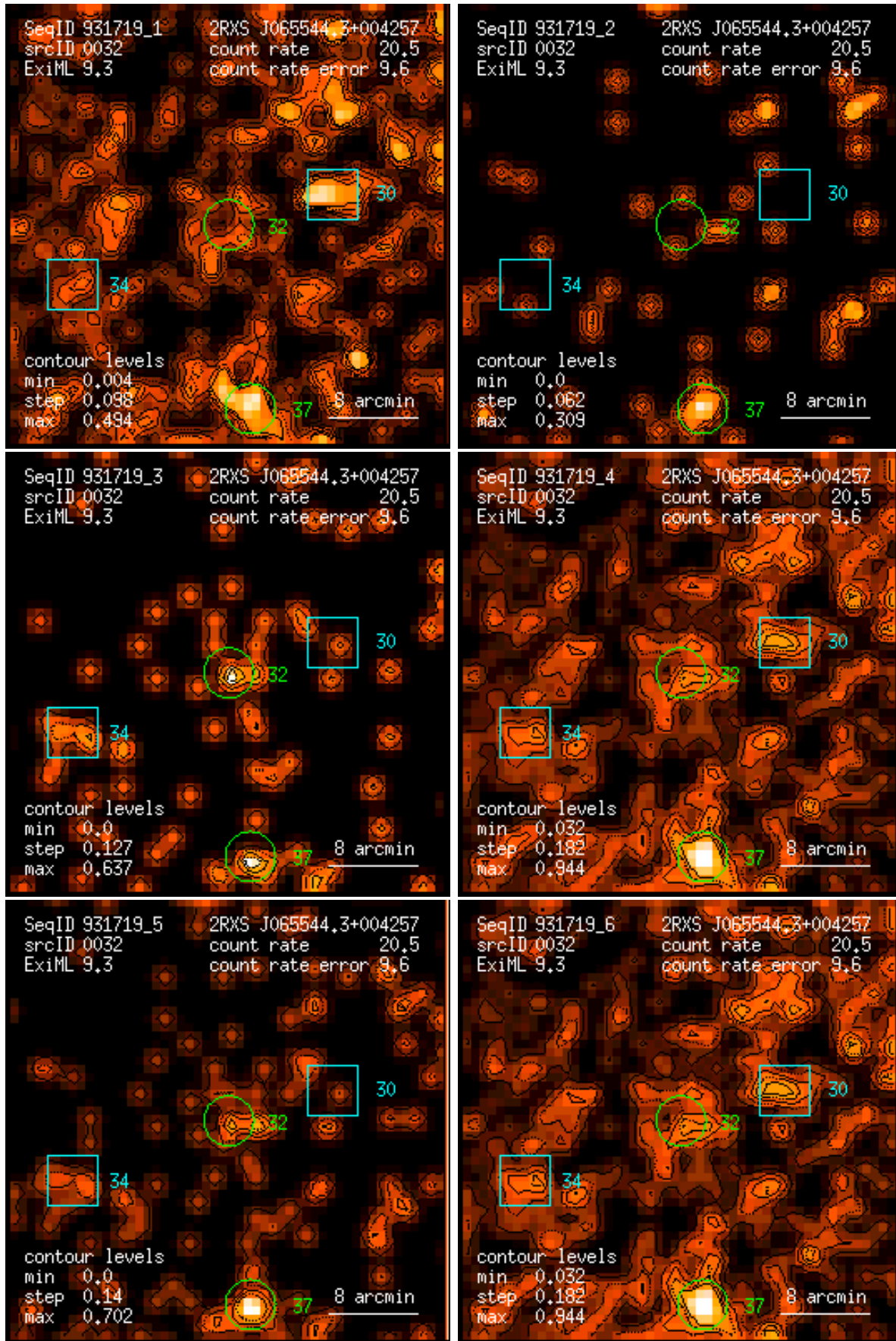
Figure 32: RASS 931719: detection 0032: band rate images, Gaussian filter: (1) PSPC channels 11 – 41, (2) 52 – 90, (3) 91 – 201, (4) 11 – 235, (5) 52 – 201, (6) 11 – 201. Broad band rates in counts/ks. Band rate contour levels in counts/ks/arcmin 2 .
