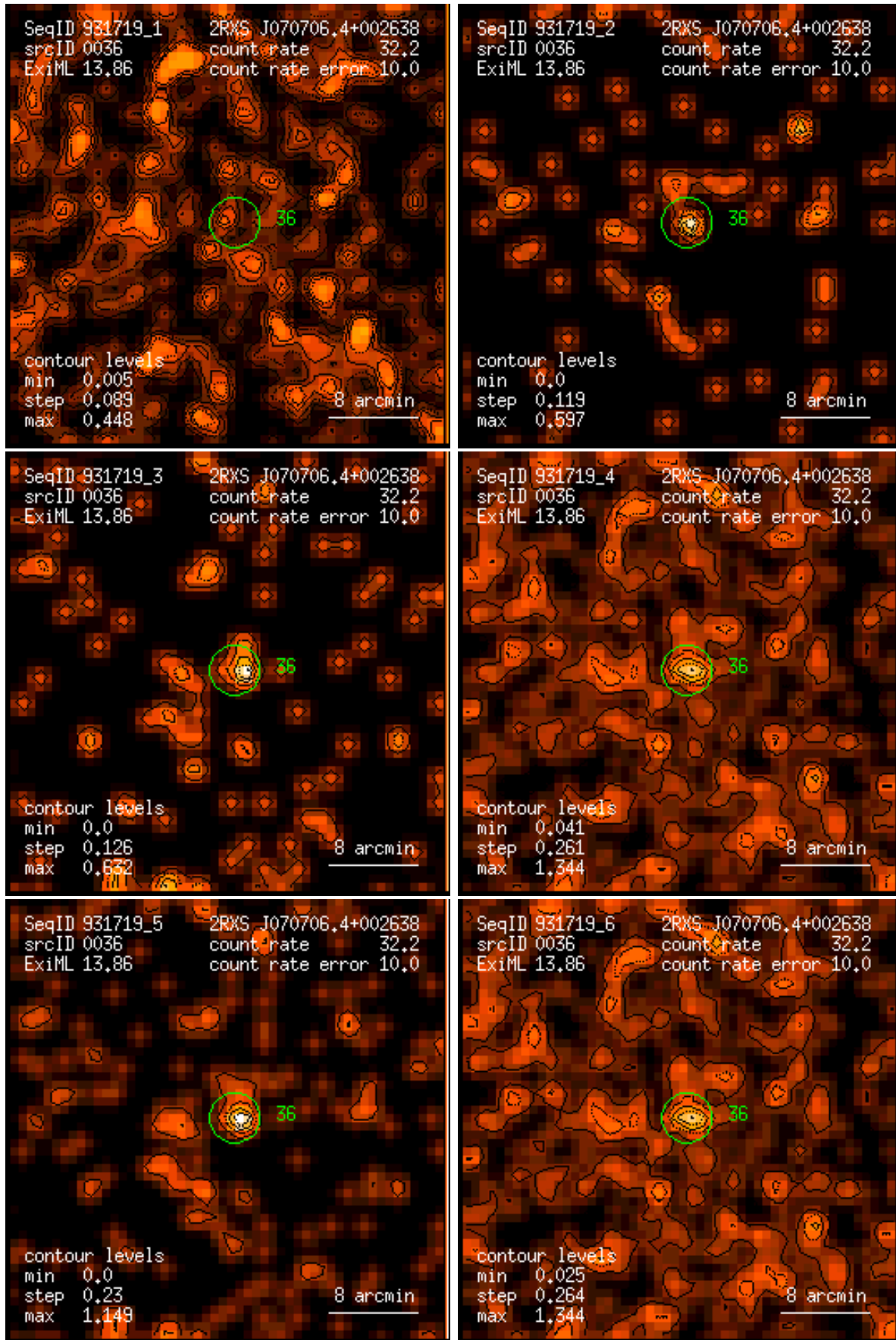
Figure 36: RASS 931719: detection 0036: band rate images, Gaussian filter: (1) PSPPC channels 11 – 41, (2) 52 – 90, (3) 91 – 201, (4) 11 – 235, (5) 52 – 201, (6) 11 – 201. Broad band rates in counts/ks. Band rate contour levels in counts/ks/arcmin 2 .
