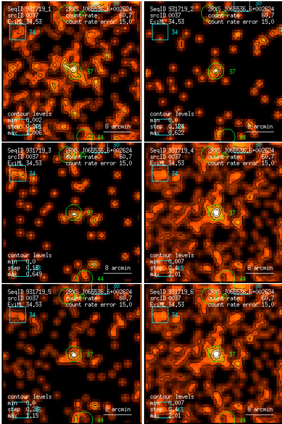
Figure 37: RASS 931719: detection 0037: band rate images, Gaussian filter: (1) PSPC channels 11 – 41, (2) 52 – 90, (3) 91 – 201, (4) 11 – 235, (5) 52 – 201, (6) 11 – 201. Broad band rates in counts/ks. Band rate contour levels in counts/ks/arcmin 2 .
