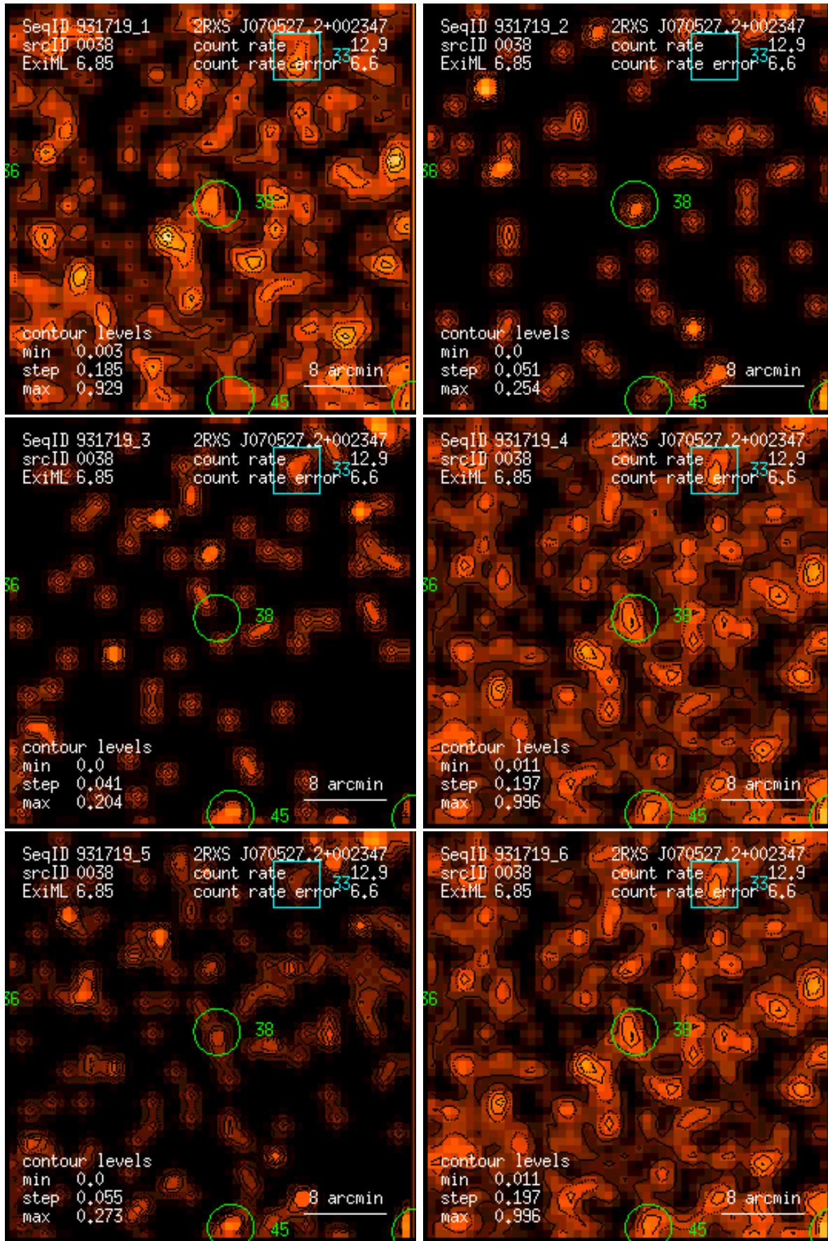
Figure 38: RASS 931719: detection 0038: band rate images, Gaussian filter: (1) PSPC channels 11 – 41, (2) 52 – 90, (3) 91 – 201, (4) 11 – 235, (5) 52 – 201, (6) 11 – 201. Broad band rates in counts/ks. Band rate contour levels in counts/ks/arcmin 2 .
