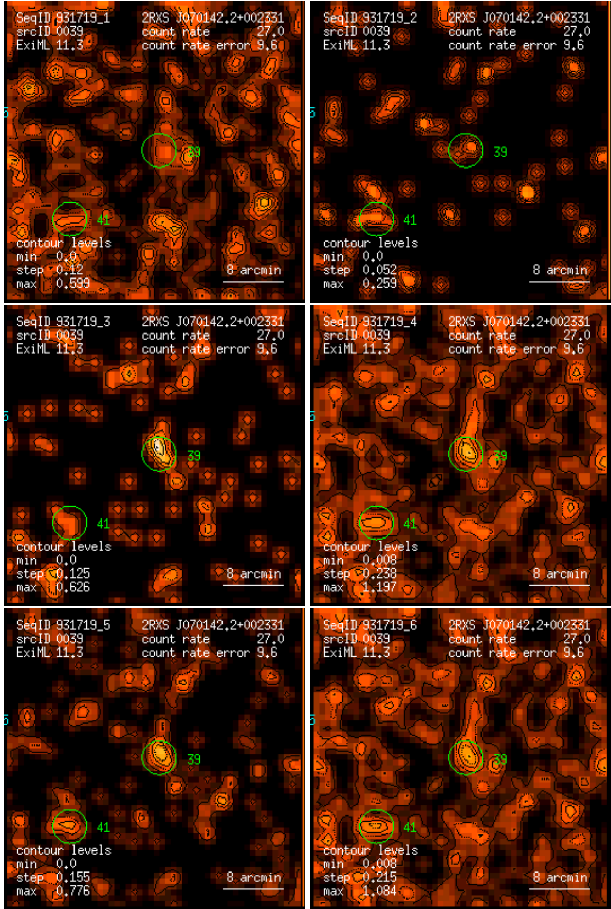
Figure 39: RASS 931719: detection 0039: band rate images, Gaussian filter: (1) PSPC channels 11 – 41, (2) 52 – 90, (3) 91 – 201, (4) 11 – 235, (5) 52 – 201, (6) 11 – 201. Broad band rates in counts/ks. Band rate contour levels in counts/ks/arcmin 2 .
