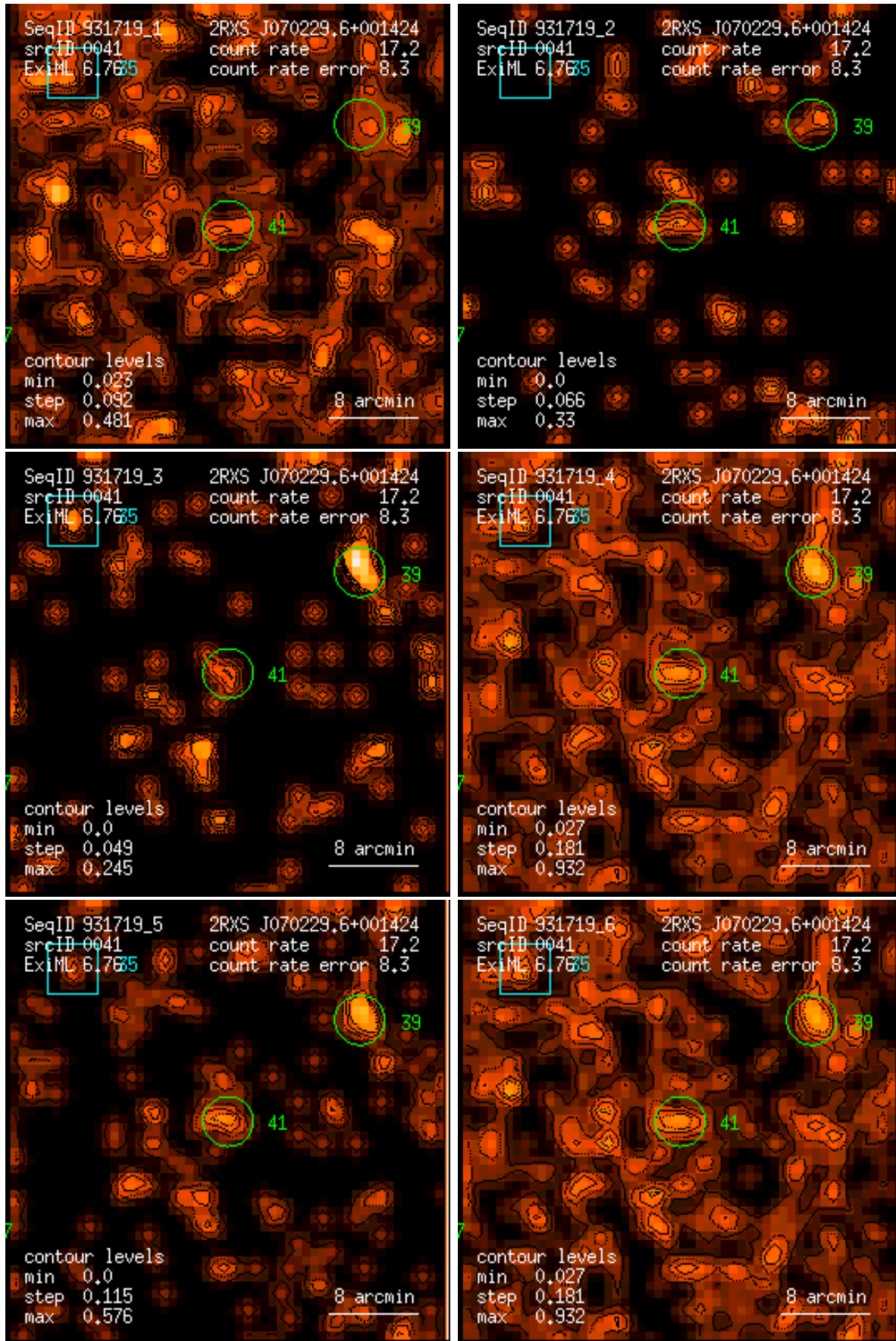
Figure 41: RASS 931719: detection 0041: band rate images, Gaussian filter: (1) PSPC channels 11 – 41, (2) 52 – 90, (3) 91 – 201, (4) 11 – 235, (5) 52 – 201, (6) 11 – 201. Broad band rates in counts/ks. Band rate contour levels in counts/ks/arcmin 2 .
