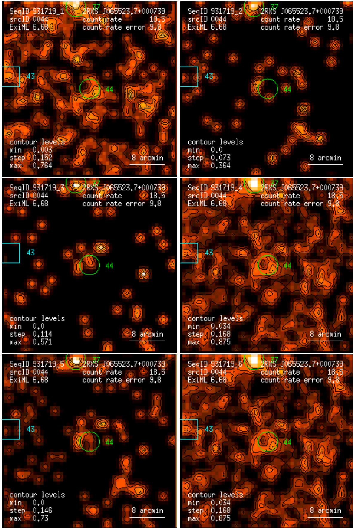
Figure 44: RASS 931719: detection 0044: band rate images, Gaussian filter: (1) PSPC channels 11 – 41, (2) 52 – 90, (3) 91 – 201, (4) 11 – 235, (5) 52 – 201, (6) 11 – 201. Broad band rates in counts/ks. Band rate contour levels in counts/ks/arcmin 2 .
